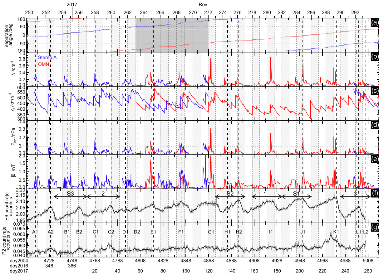
Figure 4. Plot indicating heliospheric conditions at Saturn from Day 326 of 2016 to Day 270 of 2017, spanning the Cassini F ring and proximal orbit interval (plus Rev 250). The 2016/2017 boundary is marked at the top of the figure. Also marked at the top are the times of apoapses at the start of each Rev, labeled every other Rev, with vertical alternate white/light-gray striping across all panels marking full Cassini Revs. Figures 4a–4e show solar wind/IMF parameters derived from the Tao et al. (2006) propagation model, using data from Stereo-A (blue) and OMNI (red). Figure 4a shows the data source-Sun-Saturn separation angle for each data set, where the dark-gray-shaded region between Days 55 and 121 of 2017 corresponds to the interval where the separation angles of both data sets lie outside the \pm 90^\circ range of expected approximate validity. Both (less certain) model data sets are shown in this interval. Outside this range, only those data that lie within the \pm 90^\circ uncertainty limit are plotted (both of them for a short time near the end of the interval shown). Figures 4b–4e show the model solar wind density, velocity, dynamic pressure, and IMF magnitude, respectively. In Figure 4d the horizontal dotted line at 0.1 nPa gives a rough indication of dynamic pressures producing a significant compression of Saturn’s magnetosphere. Figure 4f shows a profile of >120 MeV proton GCRs at Saturn determined from 6 hr averages of LEMMS channel E6 count rates (gray line), together with a seven-point (1.75 day) centered running average (black line). Four-Rev data intervals discussed in section 3 and the supporting information are indicated with the relevant section numbers by the horizontal arrows. Figure 4g shows 6 hr averaged and seven-point smoothed values of LEMMS channel P2 count rates presented in the same format, showing a weak response to energetic GCR protons, as for channel E6 in Figure 4f, onto which SEP proton fluxes in the energy range 2.3–4.5 MeV are superposed (see section 2.4). Assessment of the times of solar wind compressions of Saturn’s magnetosphere, to within a day or two in either direction, are shown by vertical black dashed lines. These are labeled in Figure 4g, where letters indicate events within a given solar rotation, with further information on the choice of times being given in Table 1.
