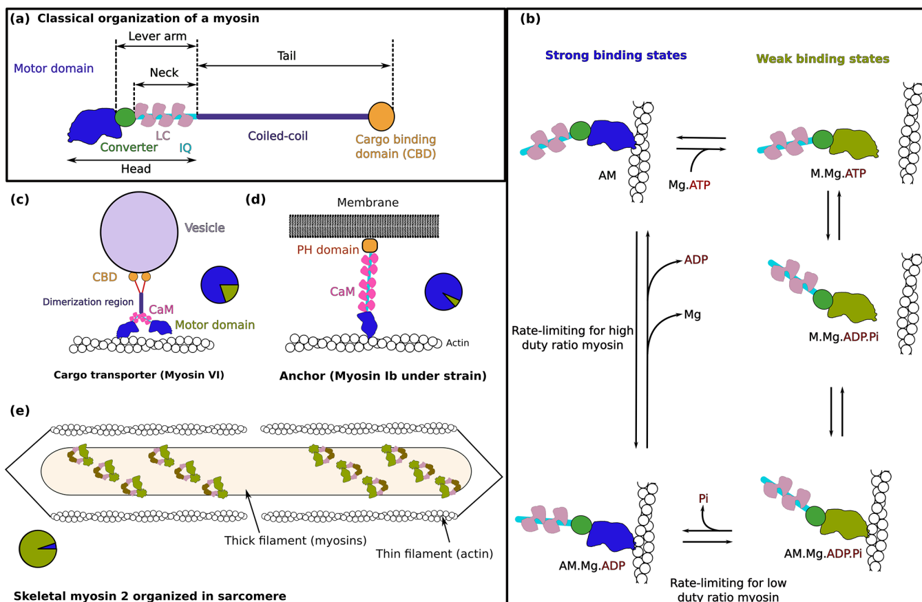
Figure 1. (a) Blueprint of a myosin. (b) Simplified representation of the ATP-dependent motor cycle of a myosin. Here the motor domains are colored depending on whether they represent weak (green) or strong (blue) binding states of the motor to actin. Depending on the rate-limiting steps within the cycle, a myosin can remain bound to actin in states of strong affinity for actin for a significant or small amount of its overall cycle (high or low duty ratio, respectively). (c–e) Examples of myosin motors with differing duty ratios. The pie chart accompanying each example represents the duty ratio by showing the ratio between weak (green) and strong (blue) binding states for actin of the overall ATPase cycle. (c) Cargo transporters, such as Myo6, are dimeric, and they are high-duty-ratio motors. (d) Myo1b functions as an anchor under strain. The motor binds lipid membranes via the tail and acts as a tension-sensitive dock or tether between the actin cytoskeleton and the membrane. (e) Organization in sarcomeres of muscle Myo2, with the heads depicted in an interacting-head motif that is found in Myo2 filaments. 10–12 These myosins are low-duty-ratio myosins.
