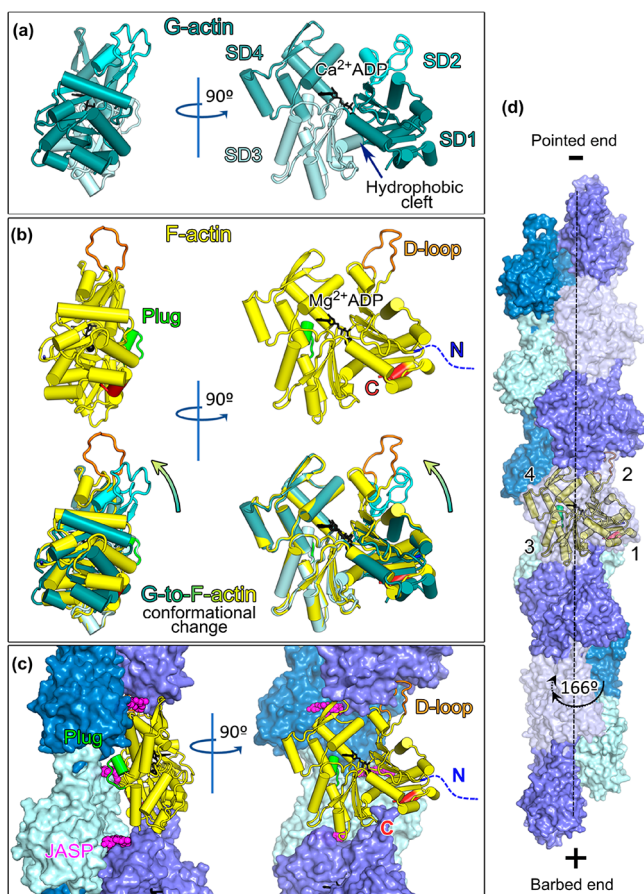
Figure 2. Actin structure. (a) Crystal structure of G-actin (PDB ID 1J6Z 34 ) in two orientations. The G-actin molecule is composed of four subdomains (SD1–SD4). A cleft between SD2 and SD4 forms the nucleotide binding pocket. The hydrophobic cleft between SD1 and SD3 is shown with an arrow. (b) Upper part , Structure of a single actin molecule within the actin filament. Lower part , Superimposition of G-actin and F-actin (PDB ID 5ONV 33 ). The structures are superimposed on SD3 and SD4. SD1 and SD2 change their orientations (shown with the arrow) upon actin incorporation into the filament. (c) The filamentous actin (F-actin) structure is stabilized by interactions between actin subunits (protomers) in a head-to-tail manner. Each actin subunit forms longitudinal contacts with two neighboring protomers. The plug is a loop connecting actin SD3 and SD4. 35,36 This structural element creates important interstrand lateral contacts with the SD1 and SD2 domains of the neighboring actin molecules within F-actin. Jasplakinolide (JASP) binds and stabilizes the lateral contacts. (d) Actin forms a double-stranded filament with 166° helical twist (arrow). Binding of partners or strain applied on the filament can modify this twist (dotted line). F-actin pointed (–) and barbed (+) ends are labeled.
