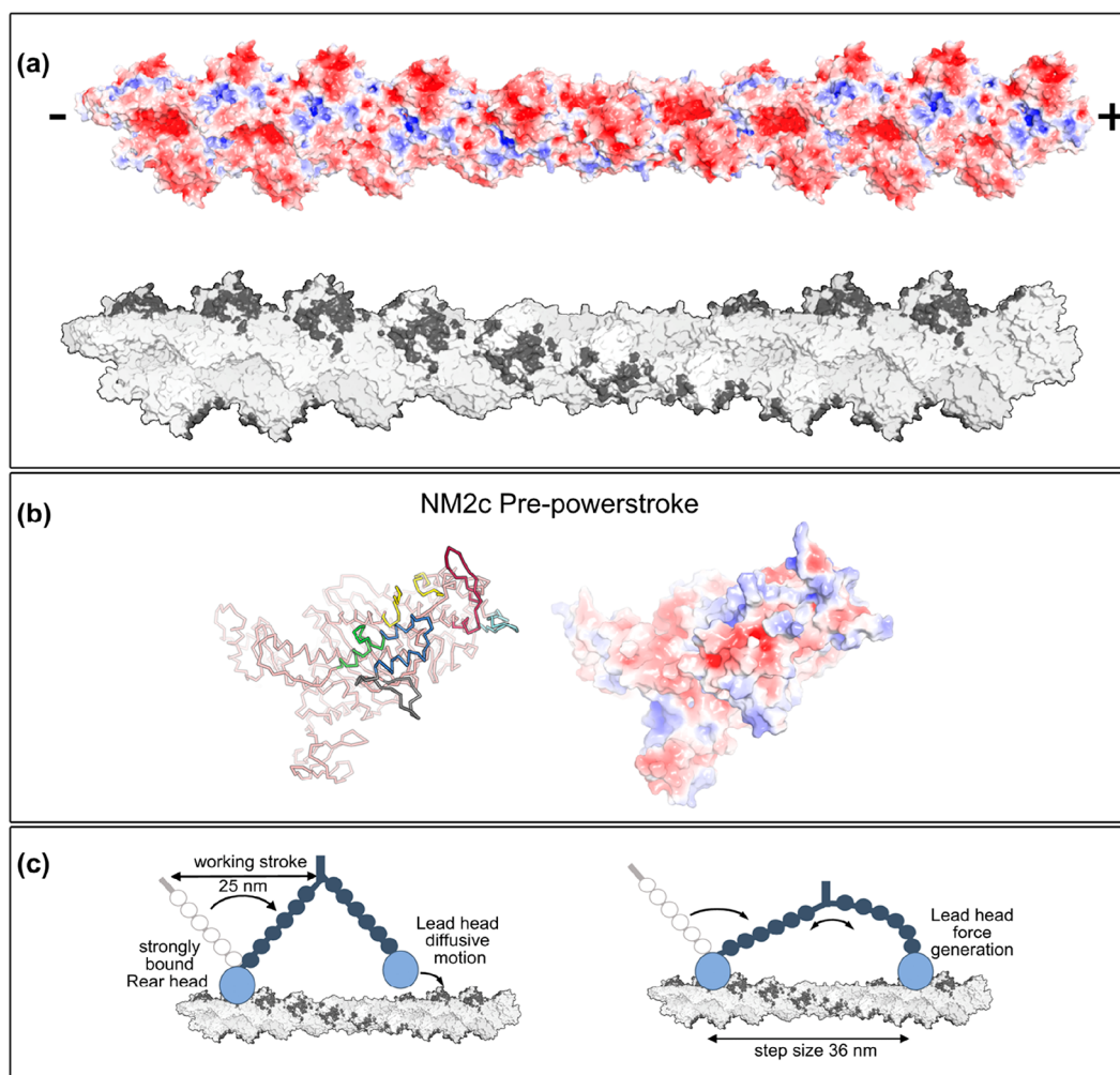
Figure 12. Distribution of the myosin binding sites on F-actin. (a) Top , F-actin surface colored by electrostatic potential distribution (red -5 ; blue 5 K_bT/e_c ). Bottom , Myosin binding sites (dark gray) are mapped on the actin filament (light gray). (b) NM2c in the Pre-powerstroke conformation (PDB ID 5I4E 66 ). Left , the actin binding elements are colored as in Figure 7. Right , the NM2c surface is colored according to the electrostatic potential distribution (red -5 ; blue 5 K_bT/e_c ). (c) Schematic drawing of two-headed Myosin V walking along F-actin. The length and flexibility of the lever arm and head/head junction permit lead head diffusion to the most favorable actin binding sites on the track.
