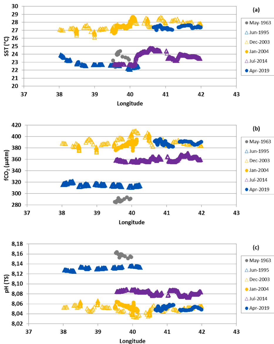
Fig. 9. Sea surface water temperature (a), f\text{CO}_2 (b) and calculated pH (c) around 25^\circ\text{S} in the Mozambique Channel observed in May 1963, June 1995, December 2003, January 2004, July 2014 and April 2019. Cruises are listed in Table 1 and tracks identified in Fig. 1. The mean observations for each cruise are listed in Table 4.
