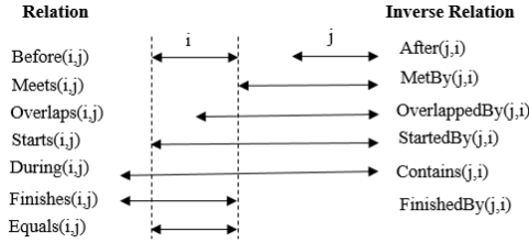
Figure 2: Allen's Relations.
