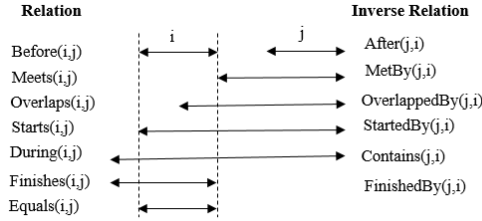
Figure 2: Allen's Relations.
