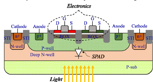
Fig. 1. A cross section of CMOS FDSOI technology. Integration of the SPAD and electronics in an inherent 3D structure with backside illumination (scales are not respected).
