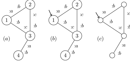
Figure 1: The different types of graphs. (a) A graph G . (b) A pointed graph (G, 1) . (c) A pointed graph modulo X .
