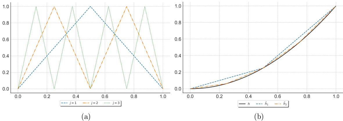
Figure 2: Plot of \psi^{[\circ j]} for j = \{1, 2, 3\} (a); approximation of h(x) = x^2 with \tilde{h}_\ell for \ell = \{1, 2\}
