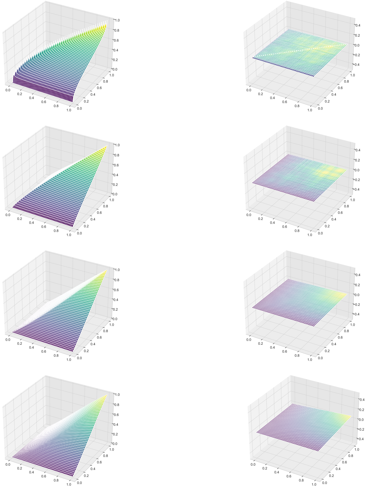
Figure 8: fBm covariance surface for H = \{0.2, 0.4, 0.6, 0.8\} presented as rows. Left: real normalized function (t, s) \mapsto V_H^{-1}\text{Cov}(B^H(t), B^H(s)) . Right: error (t, s) \mapsto V_H^{-1}(\text{Cov}(B^H(t), B^H(s)) - \text{Cov}(\tilde{B}_N^H(t), \tilde{B}_N^H(s))) for (t, s) \in [0, 1]^2 .
