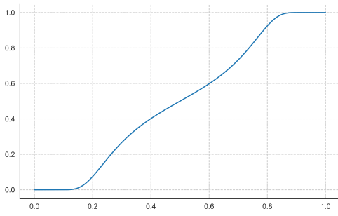
(a) u \mapsto \nu(u)
