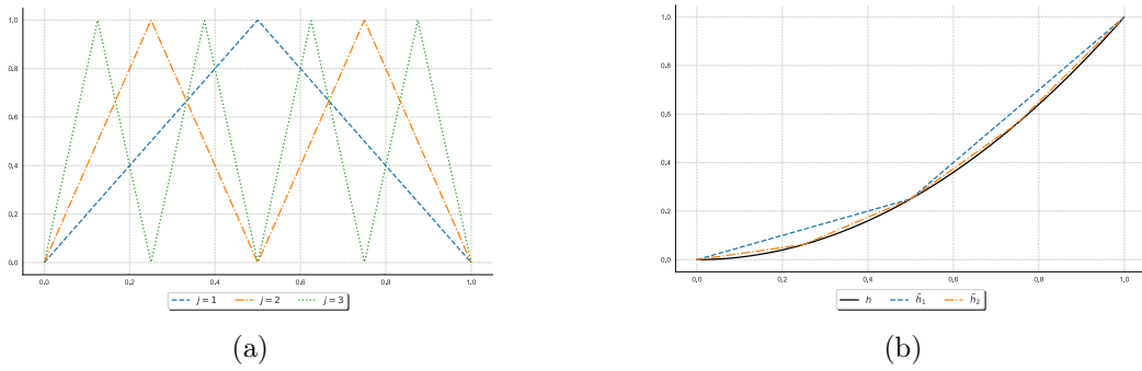
Figure 2: Plot of \psi^{[\circ j]} for j = \{1, 2, 3\} (a); approximation of h(x) = x^2 with \tilde{h}_\ell for \ell = \{1, 2\}
