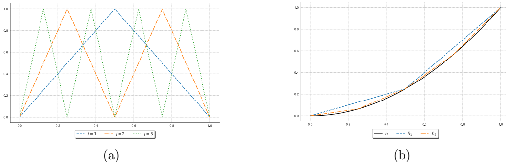
Figure 2: Plot of \psi^{[oj]} for j = \{1, 2, 3\} (a); approximation of h(x) = x^2 with \tilde{h}_\ell for \ell = \{1, 2\}
