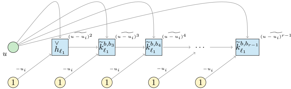
Figure 5: Neural network architecture of all power functions of (u - u_i)^q for q \in \{2, \dots, r - 1\} with b = 2\delta and b_q defined in (30).
