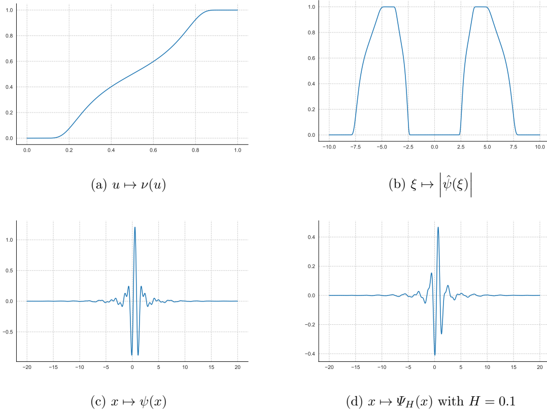
Figure 7: Lemarié-Meyer wavelet constructed with (13) for \gamma = 2
