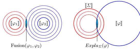
Fig. 1. Fusion based on dilations (left) and explanation based on erosions (right).
