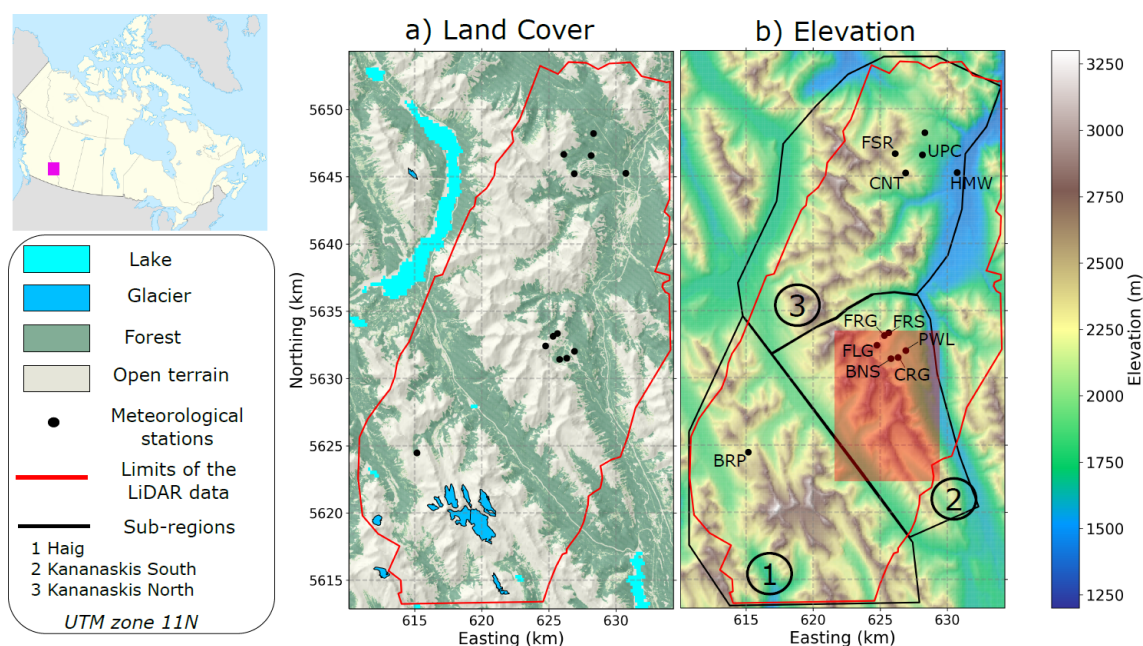
Figure 1. (a) Land cover map and (b) elevation map of the Kananaskis Valley, Alberta, Canada, study domain. The glacier mask is taken from the Randolph Glacier Inventory version 6.0 (Pfeffer et al., 2014). The red-shaded area corresponds to the area shown in Figs. 2, 3, 6 and 10. The characteristics of the meteorological stations are given in Table 3. Areas labelled from 1 to 3 correspond to sub-regions used in the analysis of the results (see Sect. 2.3.2).
