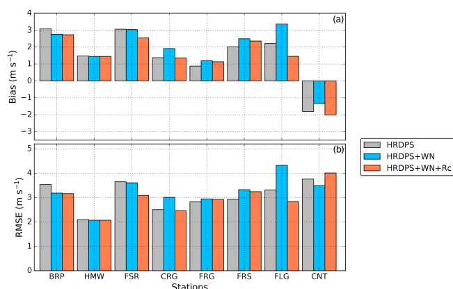
Figure 4. Evaluation of simulated wind speed using different down-scaling methods: (a) bias and (b) root-mean-square error (RMSE). Grey colours show the HRDPS wind speed without downscaling, blue colours show the HRDPS wind speed combined with Wind-Ninja microscale winds (HRDPS + WN) and red colours show the same configuration as HRDPS + WN including in addition the wind speed reduction on leeward slopes. Stations used for evaluation are classified by increasing TPI (Table 3). Their location is shown in Fig. 1.
