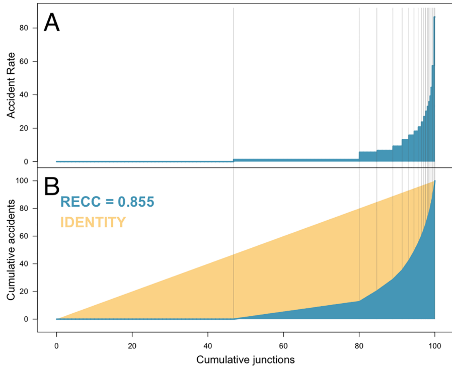
Fig 5. RECC of accidents in Central London between 2005 and 2014. A: The accident rate ( \hat{\lambda}_k ) and group sizes ( \hat{q}_j ). B: Cumulative accident rates (blue) and the Lorenz curve (in yellow). The RECC is represented by (twice) the area between the two curves.
