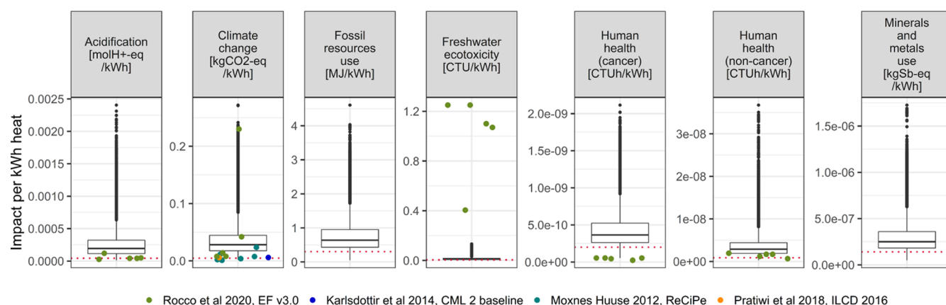
Figure 2. Comparison of the reference LCA model outcomes ( \text{Impact}_{m,i} ) (ILCD 2018) to the LCA results reported by Huuse and Moxnes, 2012; 50 Karlisdottir et al., 2014; 49 Pratiwi et al., 2018 43 (only for climate change); and Rocco et al., 2020. 40 In the boxplots, the lower and upper hinges correspond to the 25th and 75th percentiles, while the whiskers extend from the hinge to the value no further than 1.5 \times interquartile range from the hinge. The red dashed line represents the outcome of the reference LCA model using default values corresponding to the Rittersshoffen geothermal heat plant.
