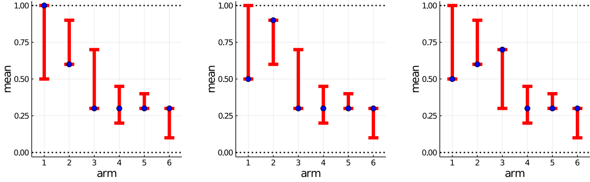
Figure 1: List of bandits (\tilde{\mu}^{\text{test}(a)})_{a \in \text{PotentialBest}} tried by Algorithm 1 for the example confidence region in red with \text{PotentialBest} = \{1, 2, 3\} . From left to right: \tilde{\mu}^{\text{test}(1)} , \tilde{\mu}^{\text{test}(2)} and \tilde{\mu}^{\text{test}(3)}
