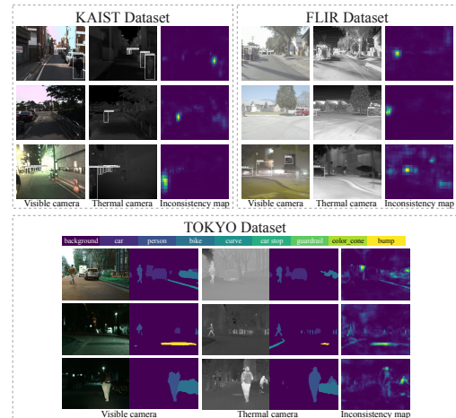
Fig. 5. Examples of selected image pairs for labelling by the proposed method. Zoom in to see details.
