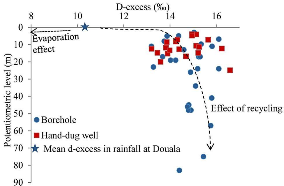
Fig. 8 Deuterium excess (D-excess) in groundwater versus potentiometric level. The mean values of D-excess in rainwater at Douala are also plotted.
