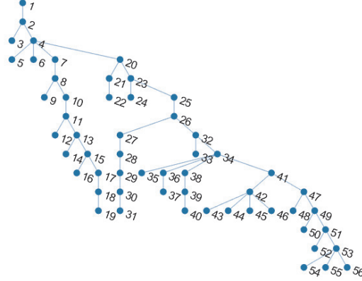
Figure 2: 56 buses network [13]
