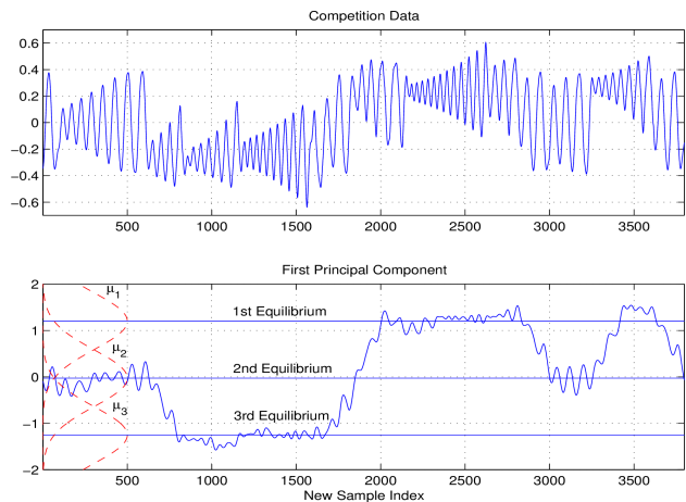
Fig. 5. Resampled Time Series, 1st Principal Component and Membership Functions.
