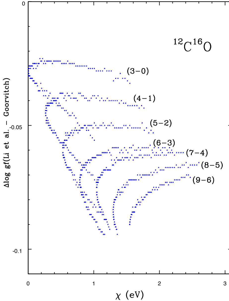
Figure 3. Comparisons of ^{12}\text{C}^{16}\text{O} gf -values between Li et al. (2015) and Goorvitch (1994), shown as \Delta \log(gf) (Li et al. - Goorvitch) as a function of excitation potential ( \chi ). The progression of vibration-rotation bands, from (3-0) to (9-6), which run across the 1.5 - 1.7 \mu\text{m} , are evident, with the differences becoming greater for the higher vibration-rotation bands.
