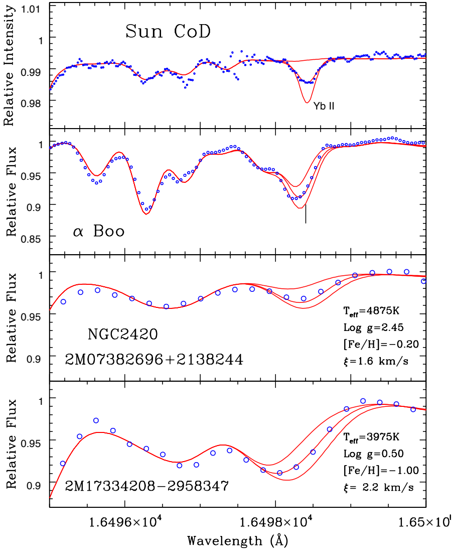
Figure 2. An illustration of the Yb II line ( \lambda 16498.42\text{\AA} ) and its behavior in four different types of stars: the Sun, the mildly metal-poor K-giant Arcturus, a clump giant in the old open cluster NGC2420, and a moderately metal-poor, cool, field red giant. The solar spectrum is Center-of-Disk (COD) from Livingston & Wallace (1991), the Arcturus spectrum is the FTS atlas from Hinkle et al. (1995), while the bottom two red giant spectra are from APOGEE. Each panel contains three synthetic spectra, with one having no Yb, another having the Yb abundance that fits the Yb II line, while a third has a Yb abundance larger by +0.2 dex compared to the best-fit abundance.
