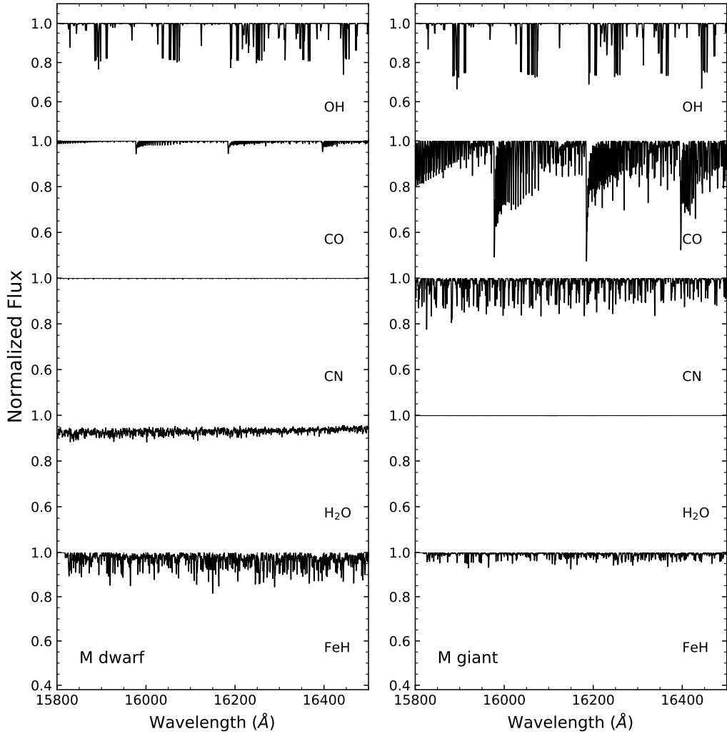
Figure 6. An illustration of absorption from the major molecular species (CO, OH, CN, H 2 O, and FeH) in typical red giant ( T_{\text{eff}} = 3800\text{K} , \log g = 1.2 , \xi = 2.0 \text{ km-s}^{-1} , [\text{Fe}/\text{H}] = 0.0 ) and M-dwarf ( T_{\text{eff}} = 3500\text{K} , \log g = 4.4 , \xi = 1.0 \text{ km-s}^{-1} , [\text{Fe}/\text{H}] = 0.0 ) spectra.
