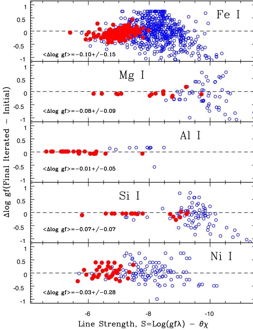
Figure 9. Differences between the final and initial log gf values ( \Delta \log gf ) for the elemental lines from Figure 8 as a function of relative line strength. Lines used to measure individual chemical abundances are plotted as filled red symbols, with these transitions representing, mostly, the stronger lines for each species ( S > -8 or -9 ), and having well-defined oscillator strengths which result in smaller iterative corrections. The weaker lines ( S < -9 ), with larger uncertainties in their oscillator strengths, have little to no impact on derived abundances. Means and standard deviations of the \Delta \log(gf) -values for lines used in abundance windows are shown for each species.
