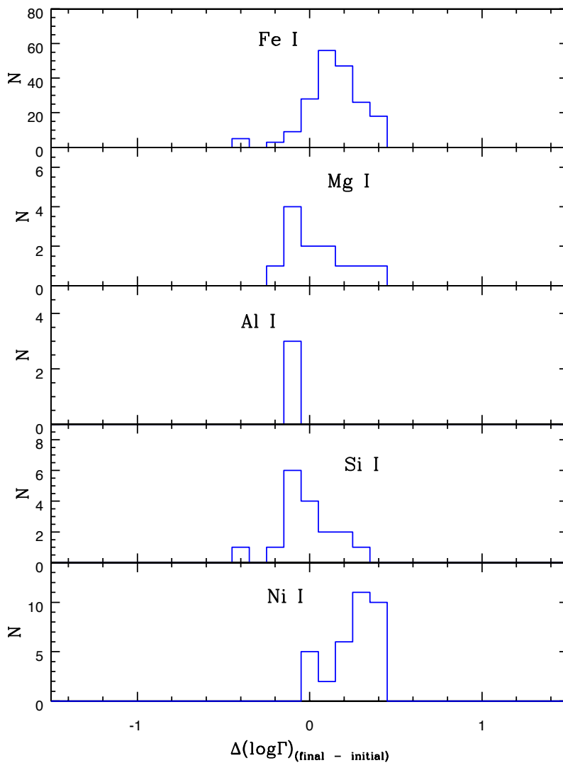
Figure 10. The difference between the astrophysically adjusted (new) and original (old) values of damping constants for lines from 5 of the major elemental species. In the APOGEE spectral window, the Mg I, Al I, and Si I lines are typically stronger than the Fe I and Ni I lines and it is worth noting that the \Delta(\log\Gamma) values for Mg I and Si I scatter about zero (Al I, with only 3 lines, is not considered in this comparison), while the values for the (weaker) Fe I and Ni I lines are offset slightly to positive values.
