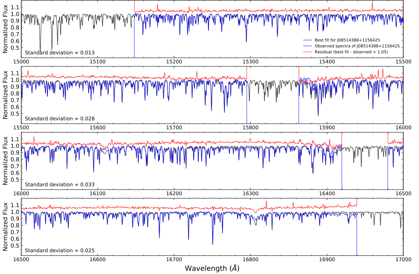
Figure 11. Synthetic spectrum computed with the DR16 line list for a red-clump star. The adopted stellar parameters are from Souto et al. (2018). The best fit synthetic spectrum is shown in black, the observed in blue, and the difference between them shown by the (shifted) red line.
