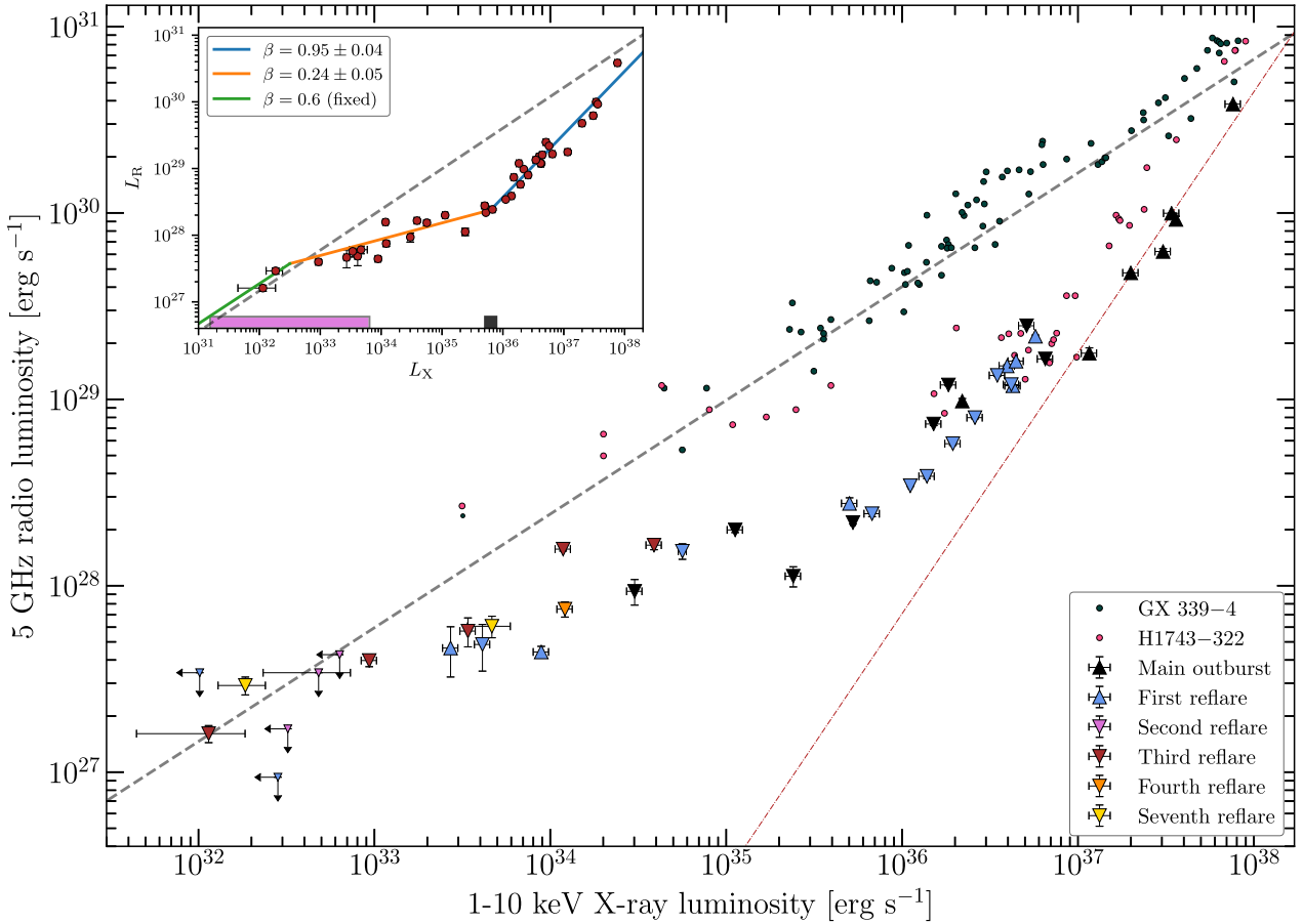
Figure 1. MAXI J1348–630 radio/X-ray diagram during its 2019/2020 outburst. We assume D = 2.2 \text{ kpc} (Chauhan et al. 2021). Points from different phases of the outburst are plotted with different colours and triangles pointing upwards or downwards differentiate between, respectively, rise and decay. The red and grey dashed lines represent, respectively, the \beta = 1.4 and \beta = 0.6 correlations (see Section 1), and are shown for illustrative purposes. The source transitions between tracks while going from higher to lower luminosities. For comparison, H1743–322 (Coriat et al. 2011) and GX 339–4 (Corbel et al. 2013; Tremou et al. 2020) are shown on the diagram with smaller size points. A tentative fit to the same data is shown in the inset in the top-left corner. The magenta and grey rectangles represent the lower and upper bounds on the x -axis of, respectively, the L_{\text{stand}} and L_{\text{trans}} confidence intervals (see Section 3).
