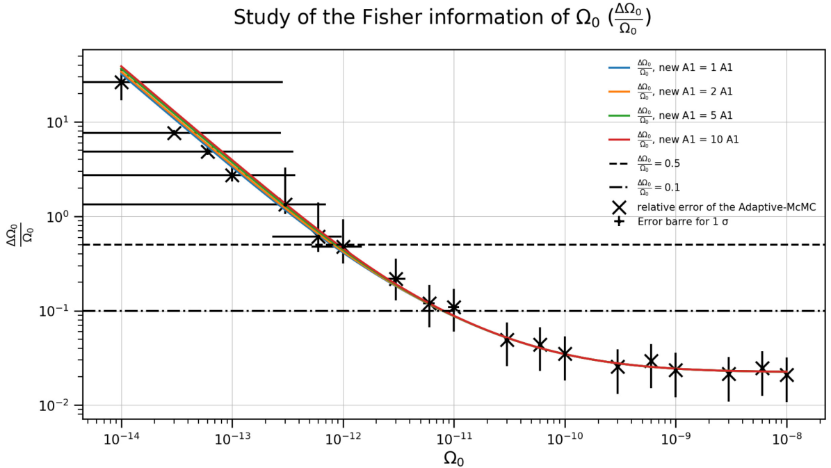
Figure 21. Uncertainty estimation of the cosmologically produced SGWB from the Fisher information study (represented as the coloured lines for four different amplitudes A_1 ) and the parameter estimation from the A-MCMC (in scatters) for the channels A and E with the noise channel T . The upper horizontal dashed line represents the error level 50 per cent. Above the line the error is greater than 50 per cent. The parameter representing the magnitude of the Galactic foreground has been modified, namely A_{1,\text{new}} = d \times A_1 for d = 1, 2, 5, 10 ; see equation (26).
