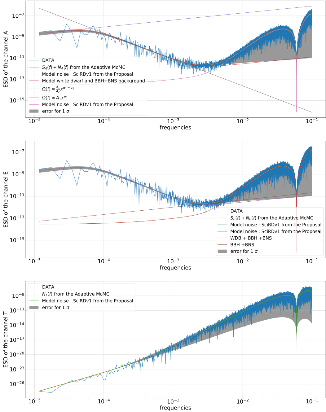
Figure 14. Energy spectral density for the channels A , E , and T from section 30 of the 50. Estimates are made for the two magnitudes of the LISA noise model from the proposal (Baker et al. 2019), the modulation of the WD foreground and the astrophysical background, with an A-MCMC of 8 parameters (BBH + DWD + LISA noise).
