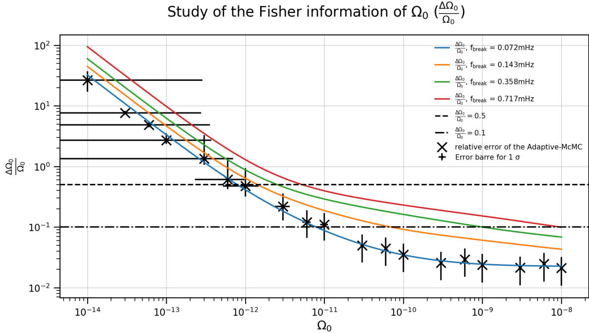
Figure 22. Uncertainty estimation of the cosmologically produced SGWB from the Fisher information study (represented as the coloured lines for four different peak frequencies in changing the spectral dependence f_{\text{break}} ) and the parameter estimation from the A-MCMC (in scatters) for the channels A and E with the noise channel T . A factor d defines a new frequency of separation of the two spectral dependencies of the Galactic foreground, f_{\text{new, break}} = d \times f_{\text{break}} . We test d = 1, 2, 5, 10 . The upper horizontal dashed line represents the error level 50 per cent. Above the line the error is greater than 50 per cent.
