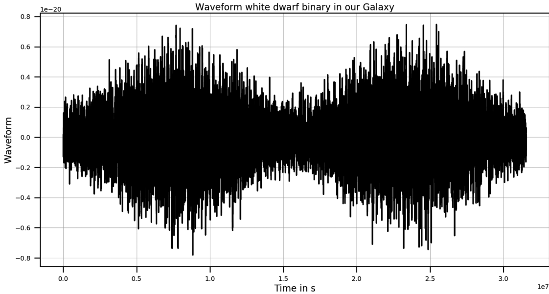
Figure 10. The total waveform, namely the sum of the five waveforms seen in Fig. 9, for the population from Lamberts et al. (2019) to be seen by LISA .
