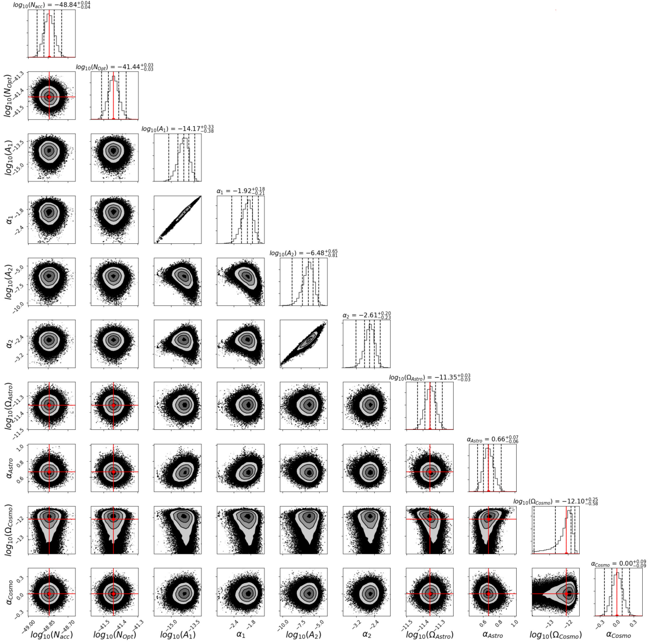
Figure 19. Corner plot for the A-MCMC of 10 parameters (BBH/BNS + WD (total waveform of 1 yr data seen by LISA ) + cosmo + LISA noise) using the channels A , E , and T . The results are for the two magnitudes for the LISA noise model from the proposal (Baker et al. 2019), and two power-law SGWB (amplitudes and spectral slopes) and the DWD (two magnitudes and two slopes). The vertical dashed lines on the posterior distribution represent from left to right the quantiles [16, 50, 84 per cent]. The red lines are the ‘true’ parameter values.
