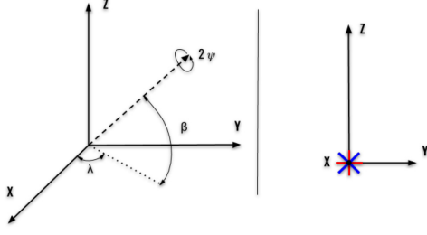
Figure 7. Generic plane waveform reference for a binary localized at ecliptic latitude \beta and longitude \lambda . The LISA constellation is in the centre of the coordinate system. We use the conventional definition from Królak, Tinto & Vallisneri (2004) for the GW polarizations: + (in red) and \times (in blue). The coordinate \Psi is the rotation around the direction of wave propagation.
