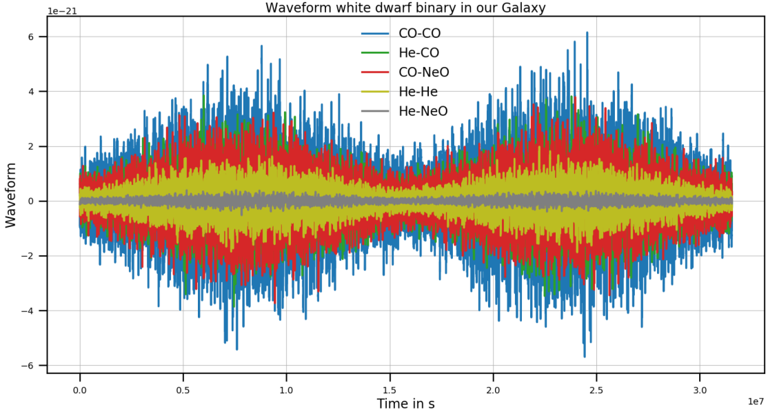
Figure 9. GW signals from the DWD modulation to be seen by LISA . The modulation is from the evolution of the orientation of the LISA constellation. The waveform s(t) is the sum of the two polarizations A = [ \times, + ] weighted by the respective detector response function F^A(\Omega, f, t) , such as s(t) = \sum_N F^\times(\Omega, f, t)h_\times(f, t) + F^+(\Omega, f, t)h_+(f, t) .
