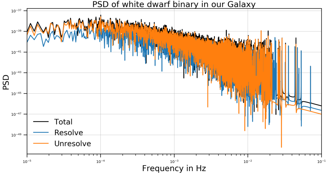
Figure 6. PSD of the GW signal for the WD binary modulation seen by LISA (see Fig. 9). The set of binaries is in black, while the resolved and unresolved are, respectively, in blue and orange. These are the same as the Fig. 4.
