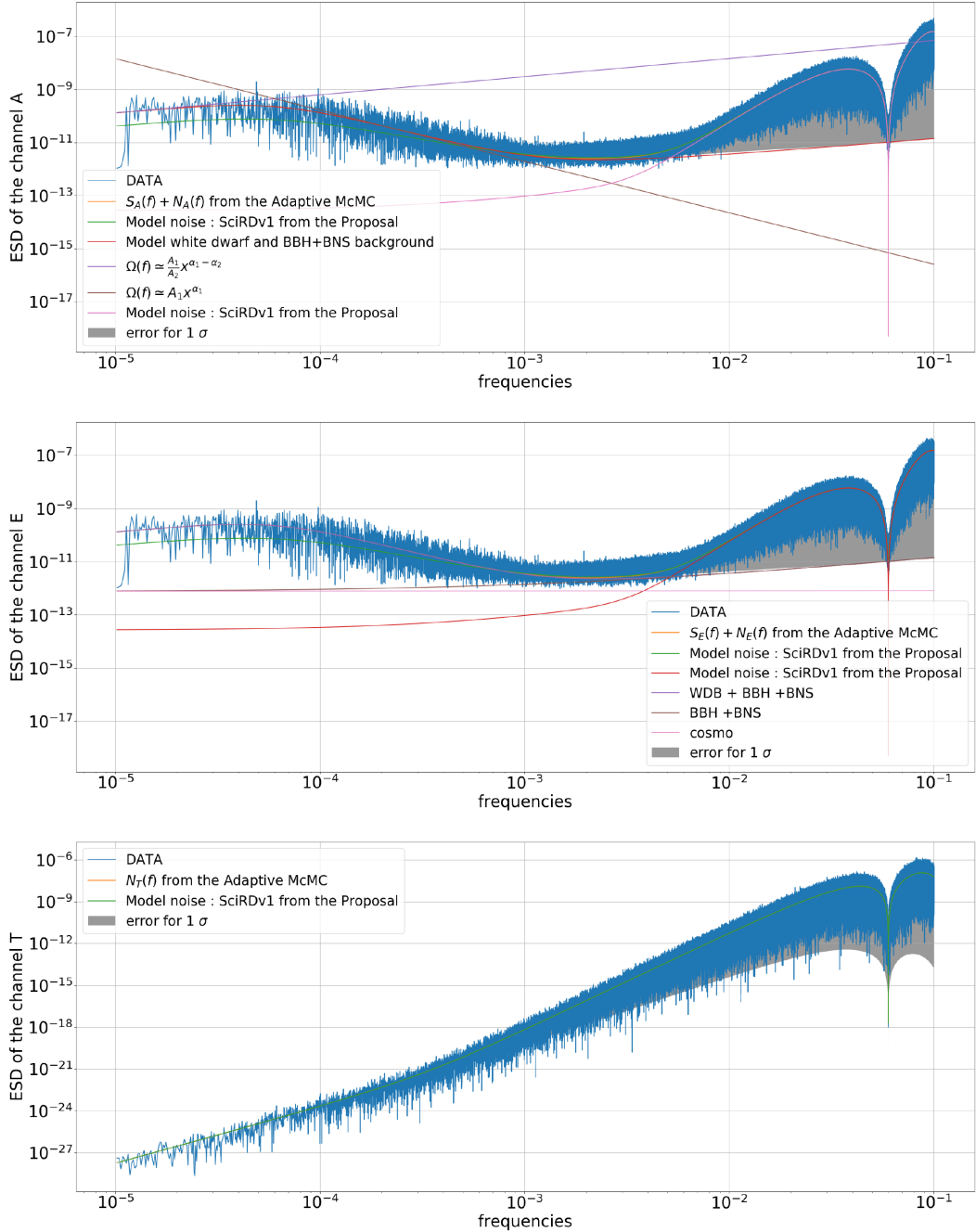
Figure 18. Energy spectral density for the channels A , E , and T from the total waveform of 1 yr data seen by LISA . Estimates are made for the two magnitudes of the LISA noise model from the proposal (Baker et al. 2019), the modulation of the WD foreground, the astrophysical background and a cosmological background with an A-MCMC of 10 parameters (cosmological + BBH + DWD + LISA noise).
