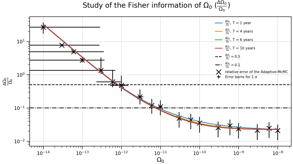
Figure 20. Uncertainty estimation of the cosmologically produced SGWB from the Fisher information study (represented as the coloured lines for four different observational time durations) and the parameter estimation from the A-MCMC (in scatters) for the channels A and E with the noise channel T . The upper horizontal dashed line represents the error level 50 per cent. Above the line the error is greater than 50 per cent.
