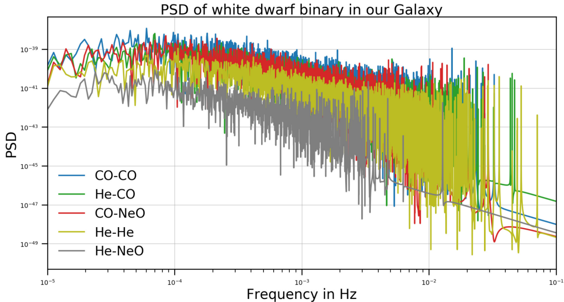
Figure 11. PSD of the GW signal for the WD binary modulation seen by LISA , (see Fig. 9). The set of binaries in blue, green, red, yellow, and grey are, respectively, the different cores CO-CO, He-CO, CO-NeO, He-He, and He-NeO. This is the direct periodogram of Fig. 9.
