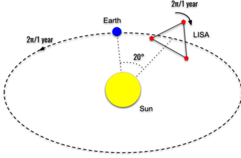
Figure 3. LISA constellation of three spacecraft. They will be placed in a heliocentric orbit and form an equilateral triangle of 2.5 million kilometer arm length. Each satellite's distance to another will be measured by laser beams. The constellation's orbit forms an angle of delay of 20^\circ with respect to that of the Earth's. Just as LISA makes an orbit of period 1 yr, during this time, it also performs a revolution on itself.
