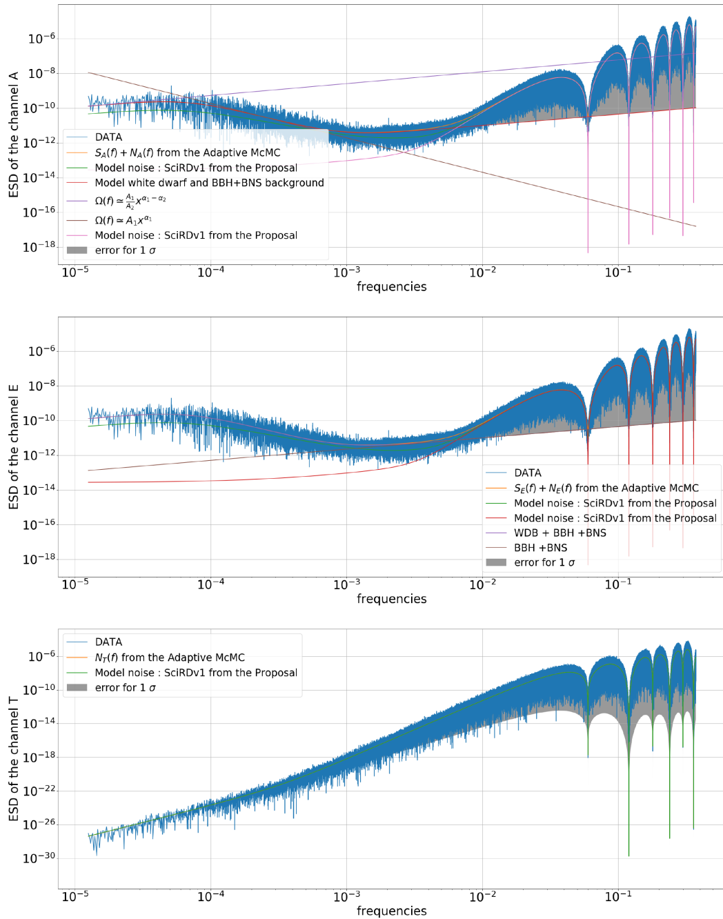
Figure 16. Energy spectral density for the channels A , E , and T from the total waveform. Estimates are made for the two magnitudes of the LISA noise model from the proposal (Baker et al. 2019), the modulation of the WD foreground, and the astrophysical background with an A-MCMC of 8 parameters (BBH + WD + LISA noise). 1 yr of data was used.
