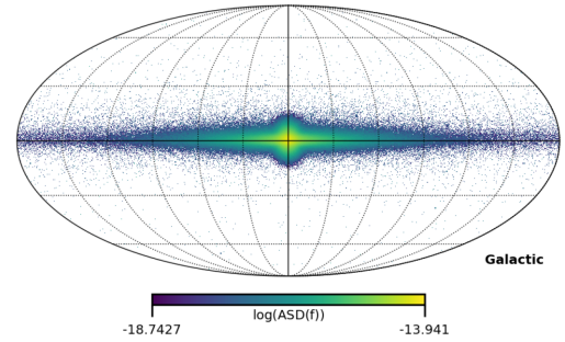
Figure 2. Map of the distribution of the log-amplitude of the GW from the Galactic WD binaries for f_{\text{GW}} \geq 1 \times 10^{-4} Hz. The DWD distribution is from the population presented in Nelemans et al. (2001).
