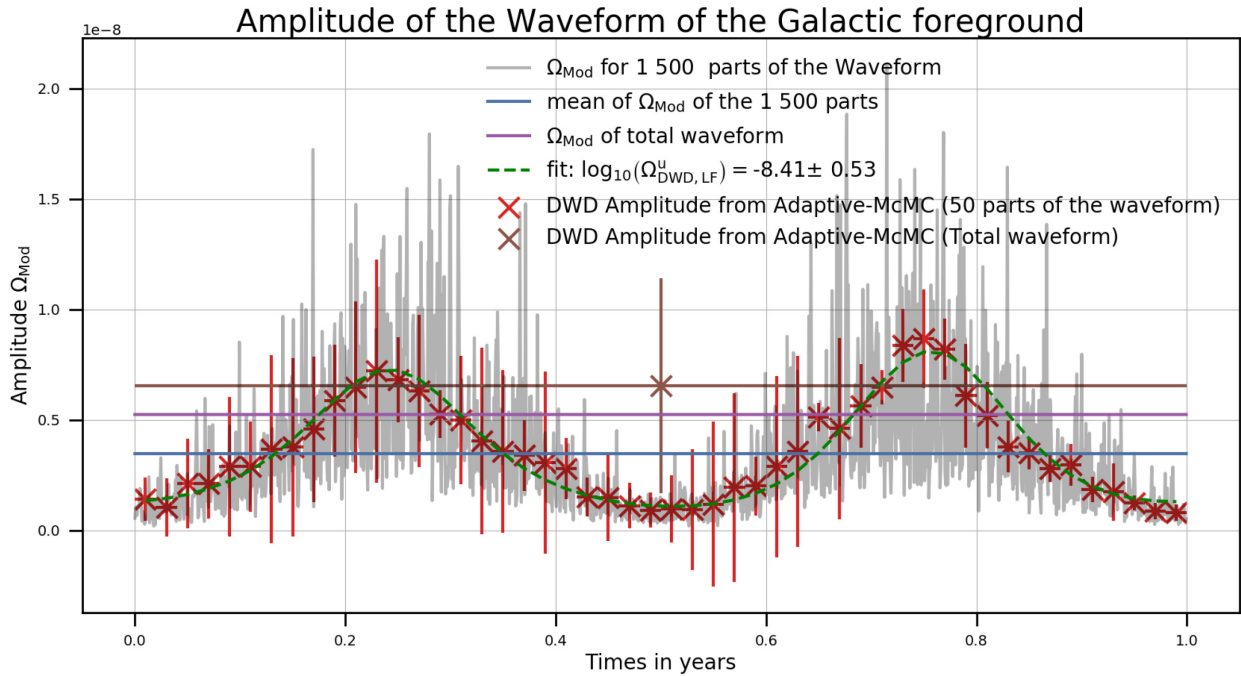
Figure 13. Measurement of the orbital modulation of the DWD amplitude. In grey: 1500 estimations of the amplitude \Omega_{\text{Mod},i} = \frac{4\pi^2}{3H_0^2} \left(\frac{c}{2\pi L}\right)^2 A_i^2 , where A_i is the amplitude of the characteristic strain of the section h_i of the waveform. The blue line is the mean of the 1500 estimations of the amplitude. In purple, the amplitude \Omega_{\text{Mod}} for the total waveform (1 year duration). This corresponds to the estimation of the amplitude of the energy spectral density of the DWD, but expressed as a time-series. In red scatter: 50 A-MCMC generated DWD amplitudes calculated from the estimates of the 8 parameters (BBH + WD + LISA noise). In brown scatter, the estimation of the amplitude energy spectral density of the Galactic foreground at low frequency with the adaptive MCMC. We also fit the 50 A-MCMC with a least squares method to estimate the modulation from the LISA antenna pattern and the ‘real’ amplitude of the Galactic foreground at low frequencies \log_{10}(\Omega_{\text{DWD,LF}}^u) = -8.41 \pm 0.53 (see equation 48) for a reference frequency (see equation 31) of 3 \times 10^{-3} Hz*(green dashed line).
