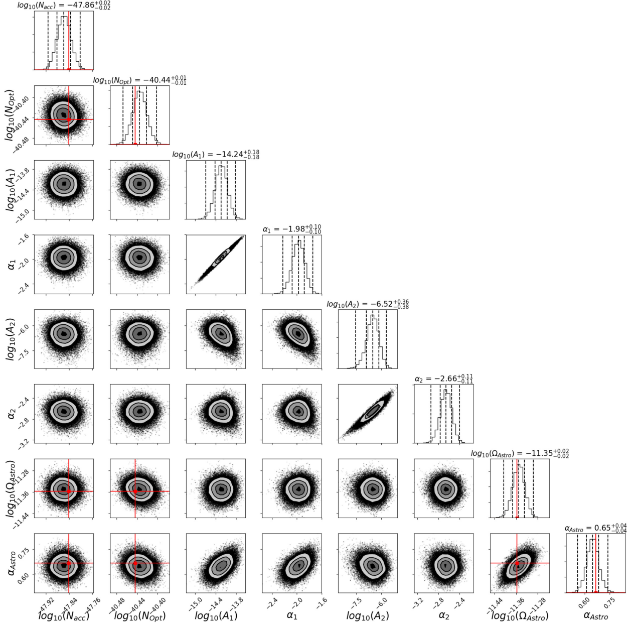
Figure 17. Corner plot for the A-MCMC of 8 parameters (BBH/BNS + WD + LISA noise) using the channels A , E , and T with 1 yr of data. The results are for the two magnitudes for the LISA noise model from the proposal (Baker et al. 2019), one single power law SGWB (amplitudes and spectral slopes) and the DWD (two magnitudes and two slopes). The vertical dashed lines on the posterior distribution represent from left to right the quantiles [16, 50, 84 per cent]. The red lines are the ‘true’ parameter values.
