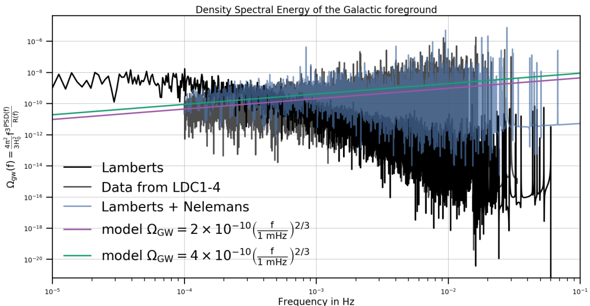
Figure 12. Normalized energy spectral density of the Galactic foreground \Omega_{\text{GW,DWD}} for different population models of DWD in the Milky Way. The black line is the Lamberts et al. population, the grey line corresponds to the population of LDC (LDC1-4); this population can be fit by a power law, see the purple line ( \Omega_{\text{GW}}(f) = 2 \times 10^{-10} \left(\frac{f}{1 \times 10^{-3} \text{ Hz}}\right)^{2/3} ). In blue, labelled by Lamberts + Nelemans, is a population generated with binaries where the Galactic spatial positions are given by Nelemans et al., and the other parameters from Lamberts et al.. This ‘Lamberts + Nelemans’ population can be fit by a power law \Omega_{\text{GW}}(f) = 4 \times 10^{-10} \left(\frac{f}{1 \times 10^{-3} \text{ Hz}}\right)^{2/3} in the frequency band [1 \times 10^{-4}, 1 \times 10^{-3} \text{ Hz}] .
