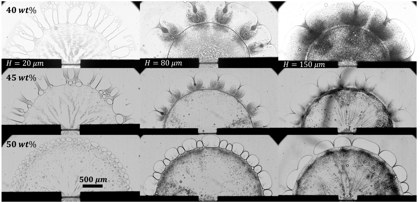
FIG. 7. Phase separation pattern at t = 50 s, for three heights of cavity H = 20, 80, and 150 \mu\text{m} (from left to right) and three compositions 40, 45 and 50 wt% (from top to bottom). The voltage is 7 Volts (80 mW).
