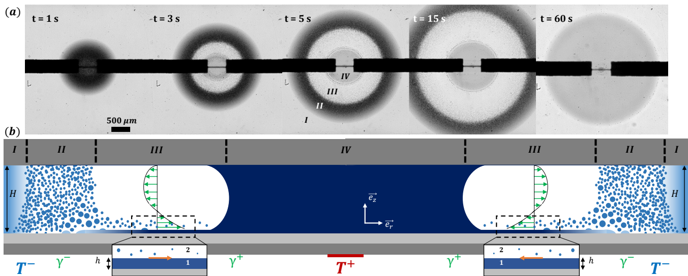
FIG. 4. (a) Top view of the separation dynamics at 7 Volts (80 mW) at different times. The mass fraction in IL is 25% and the cavity height is H = 60 \mu\text{m} . The separation dynamics can be divided into four regions, clearly visible at t = 5 \text{ s} in the top view: I) IL-water non-separated mixture, II) separation of the two phases, the droplets are mostly pushed outwards, III) some IL-rich droplets are dragged inward across the water-rich phase, IV) IL-rich sessile drop. At t = 60 \text{ s} when steady-state is reached, an IL-rich drop is accumulated above the heating resistor. (b) Cross-section sketch of the phase separation dynamics. The tread-milling wetting film induces a radial Couette-Poiseuille flow. Inset: within region III, domain 1 indicates the IL-rich wetting film and domain 2 the water-rich phase above. The orange arrows indicate the interfacial stresses.
