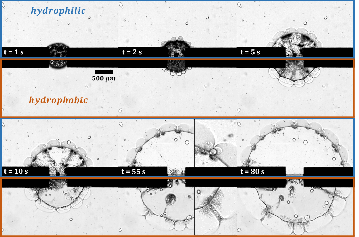
FIG. 12. Time lapse of the phase separation dynamic for two lutidine-water mixtures in two different cavities: 20wt% in lutidine for the hydrophilic cavity (oxygen plasma treated) and 40wt% in lutidine for the hydrophobic one (pristine PDMS cured at 130°C at least two hours). The lutidine-rich phase is slightly darker than the water-rich one. We recover the flower pattern formed by the periodic digitation. In the hydrophilic cavity the water-rich phase is accumulated at the center and the lutidine-rich phase gives the petals, while in the hydrophobic cavity roles are swapped. The voltage is 9.2 Volts (135 mW) and the cavity height is H = 60 \mu\text{m} . Insets: zoom on the Marangoni jets.
