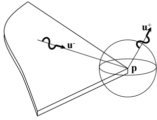
Figure 3. Diffraction of a structural ray a corner, the acoustical ray may follow any direction.
