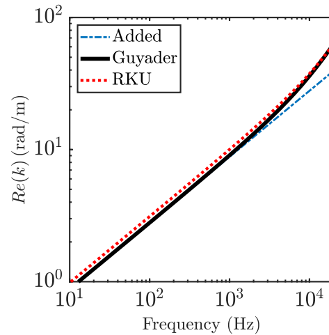
Figure 2. Wavenumbers of equivalent plate theories: sandwich plate with stiff core.
