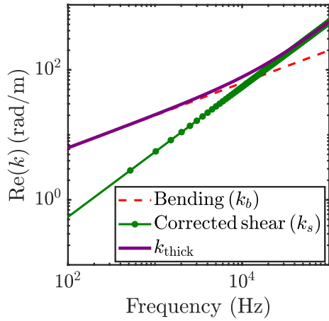
Figure 1. Propagating wavenumbers of a Reissner-Mindlin plate and its asymptotic behaviours. The plate is made of plasterboard with h = 25 mm, E = 3 GPa, \rho = 700 kg/m 3 and \nu = 0.22 .
