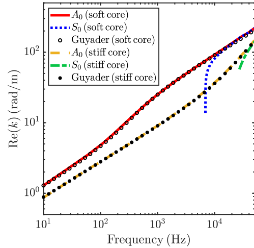
Figure 4. Anti-symmetric ( A_0 ) and symmetric ( S_0 ) wavenumbers of the first mode of a sandwich plate with soft and stiff cores, obtained from Lamb wave theory.
