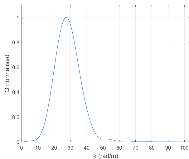
Figure 3. Q(k) , the distribution of vibrational energy versus wavenumber, at 102 Hz, normalised to its peak.
