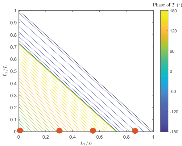
Figure 4: Phase of T as a function of L_1 and L_3 at 2000 Hz
