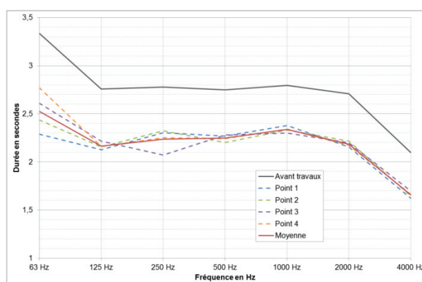
Figure 6. Measured RT_{30} in unseated, concert set-up before (black line) and after (red line, average) refurbishment
