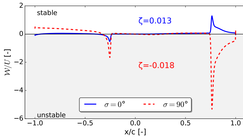
Figure 8: Extracted work along blade chord for \sigma = 0^\circ and \sigma = 90^\circ (leading edge at x/c = 0 , pressure side: x/c < 0 , suction side: x/c > 0 ) - k = 0.15
