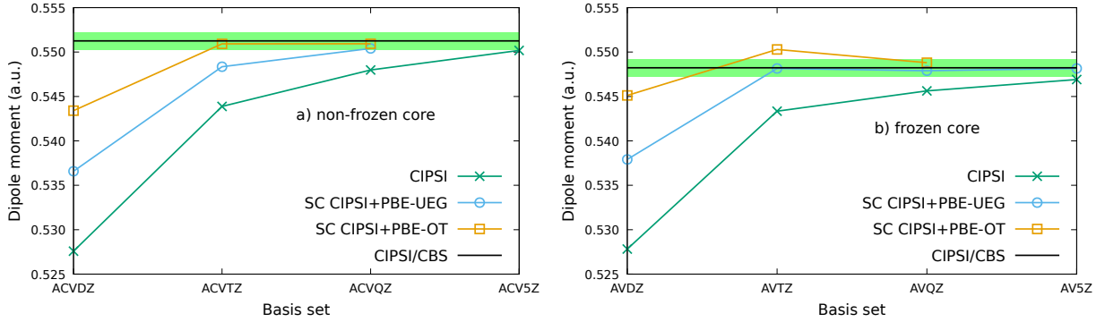
FIG. 1. Basis-set convergence of the dipole moment of the ground state of the BH molecule calculated using the aug-cc-pCVXZ (ACVXZ) and aug-cc-pVXZ (AVXZ) basis sets (with X = D, T, Q, 5 ) by CIPSI including different self-consistent basis-set corrections without the frozen-core approximation (a) and with the frozen-core approximation (b). The self-consistent basis-set corrections are for the local range-separation parameter \mu_{SD} . The green area indicates an error of \pm 0.001 a.u. around the CIPSI CBS value.
