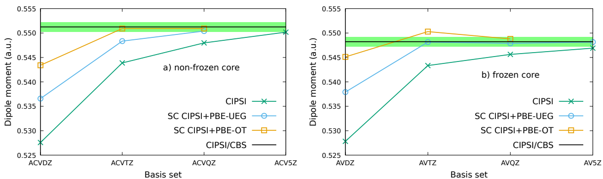
FIG. 1. Basis-set convergence of the dipole moment of the ground state of the BH molecule calculated using the aug-cc-pCVXZ (ACVXZ) and aug-cc-pVXZ (AVXZ) basis sets (with X = D, T, Q, 5 ) by CIPSI including different self-consistent basis-set corrections without the frozen-core approximation (a) and with the frozen-core approximation (b). The self-consistent basis-set corrections are for the local range-separation parameter \mu_{SD} . The green area indicates an error of \pm 0.001 a.u. around the CIPSI CBS value.
