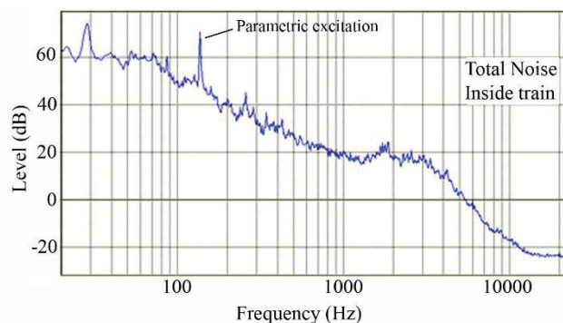
Figure 5: Spectrum of the noise measured in the lower floor of a railroad coach of a duplex TGV traveling at 300 km/h
