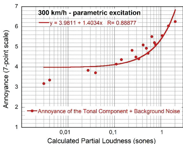
Figure 7. Annoyance as a function of partial loudness of the parametric excitation calculated with Moore et al. model [8].
