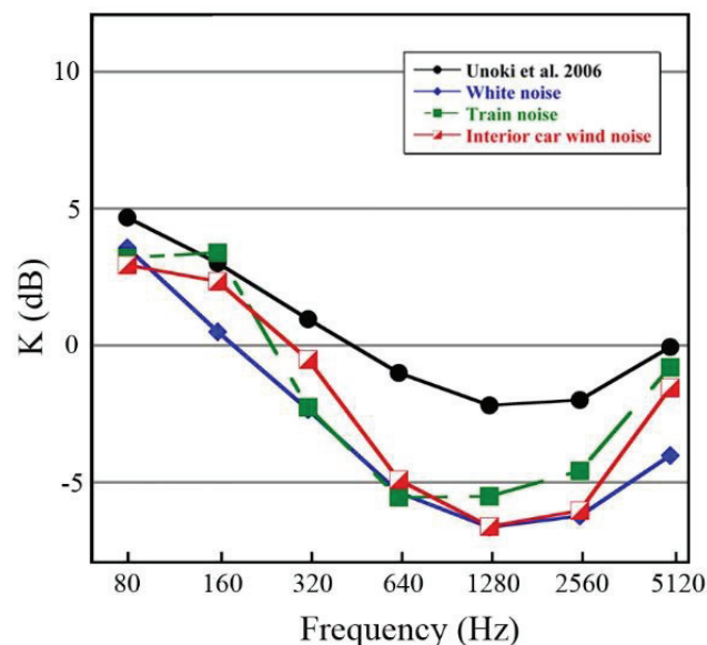
Figure 8: Parameter K, which represents the signal to masker ratio required at the output of the Roex auditory filter to reach masked threshold, as a function of the frequency of the masked pure tone, for different maskers. The maskers are: white noise (blue, diamonds), the background noise inside a train coach (green, full squares) and the aeroacoustic noise inside a car (red, semi-full squares). The black line and circles represent data adapted from Unoki et al., 2006 [27].
