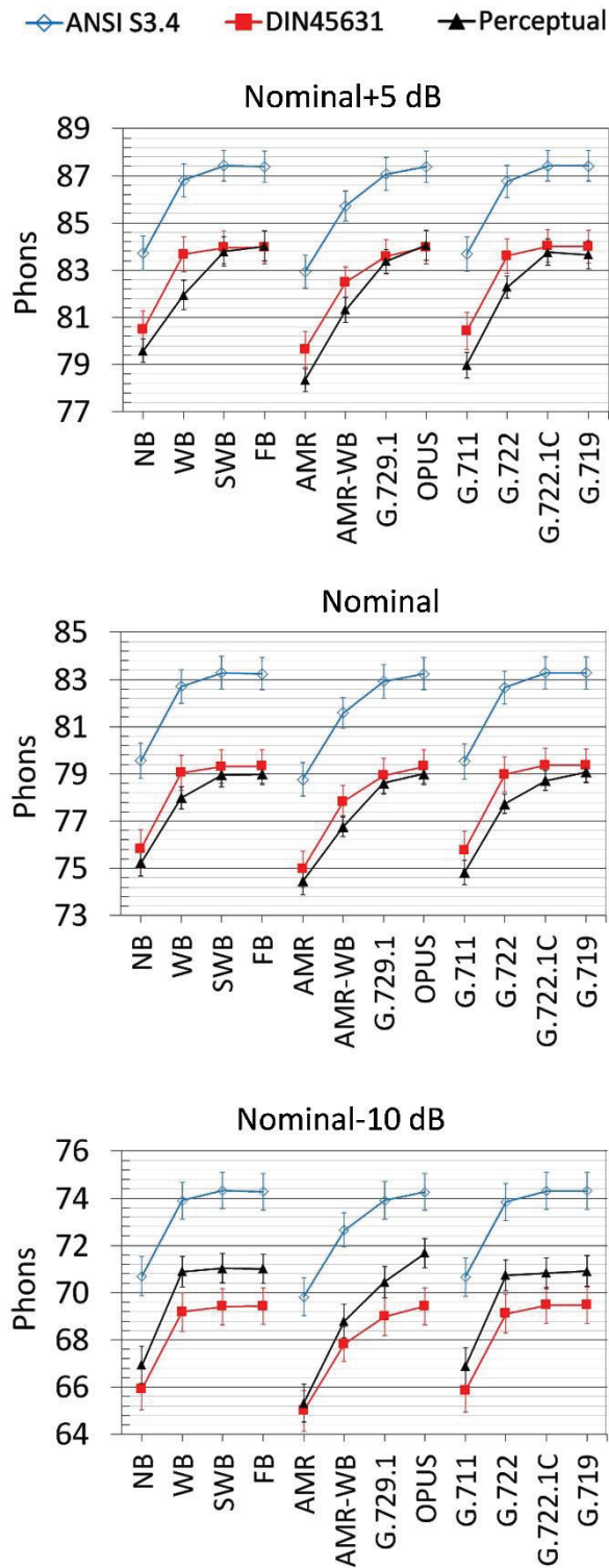
Figure 2. Loudness evaluated by listeners (Perceptual) compared to loudness calculated by models for stationary sounds (ANSI S3.4 [23] and DIN 45631 [21]), for different bandwidths and different codecs.
