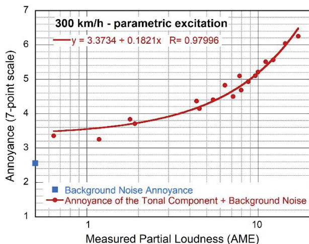
Figure 6: Annoyance as a function of measured partial loudness of the parametric excitation
