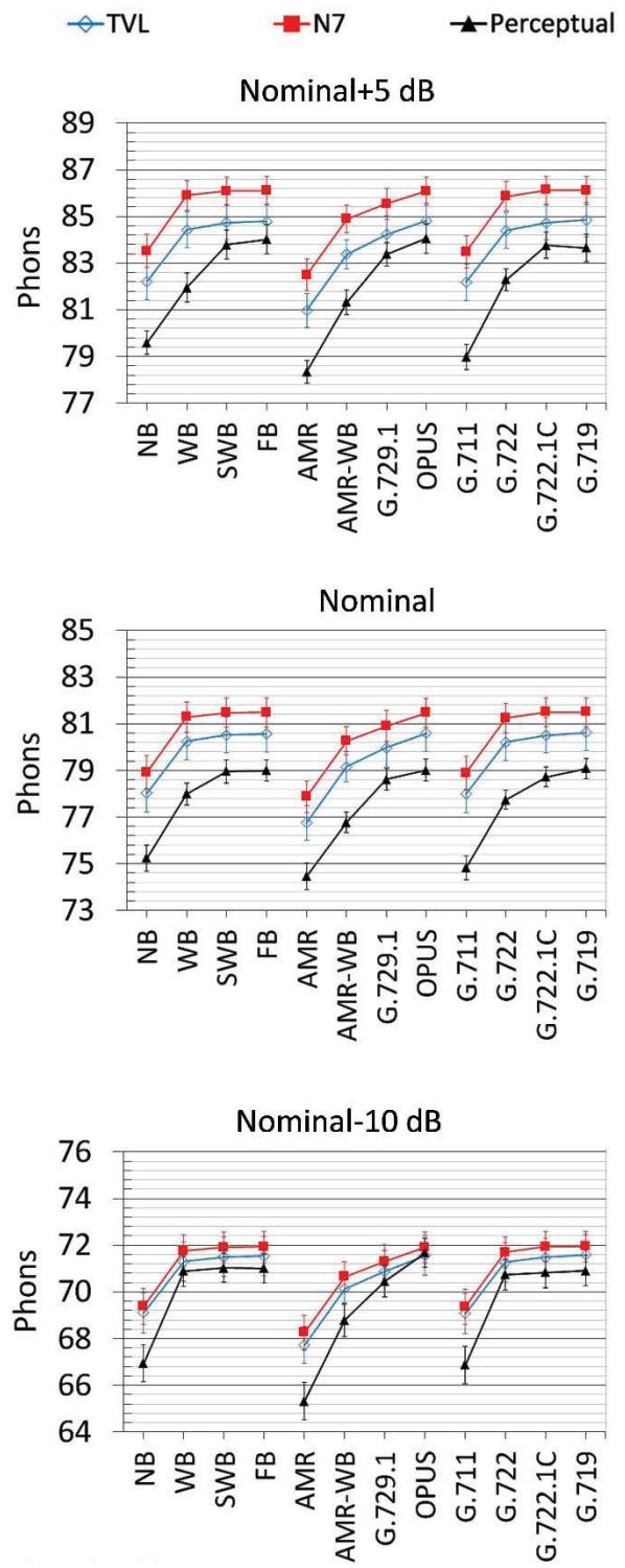
Figure 3. Loudness evaluated by listeners (Perceptual) compared to loudness calculated by models for non-stationary sounds, for different bandwidths and different codecs. TVL: averaged Long-Term Loudness [24], N7: loudness values reached and exceeded during 7 percent of the time [7].
