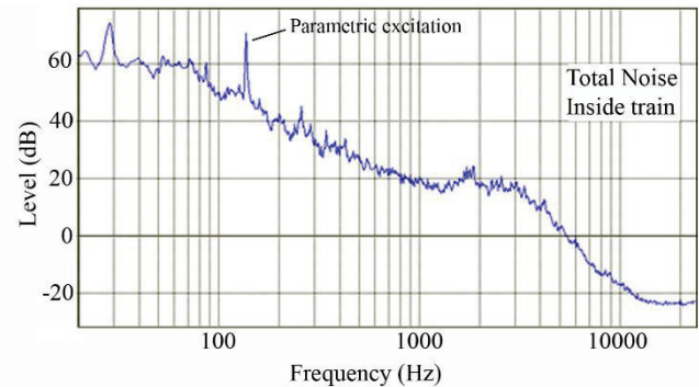
Figure 5: Spectrum of the noise measured in the lower floor of a railroad coach of a duplex TGV traveling at 300 km/h
