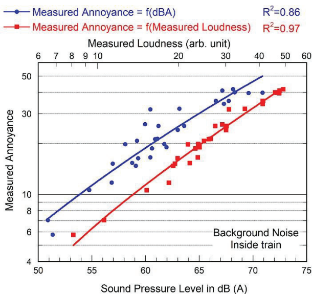
Figure 1. Annoyance as a function of dB(A) and measured loudness.
