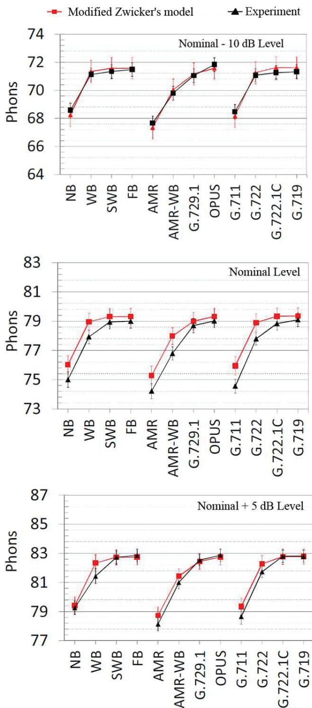
Figure 4. Loudness evaluated by listeners (Perceptual) compared to loudness calculated by the modified Zwicker's model.
