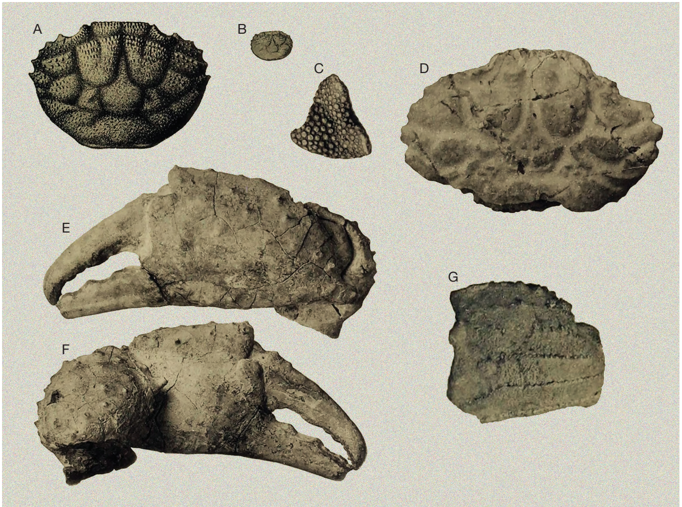
FIG. 6. — Digital reproduction of the figures from Couffon (1908) with the original nomenclature: A-D , Titanocarcinus pulchellus Al. Milne-Edwards, 1865 (sic); E, F , Cancer Sismondae Meyer, 1843? (sic); G , Cancer Deshayesii A. Milne-Edwards, 1865 (sic). Without scale.
