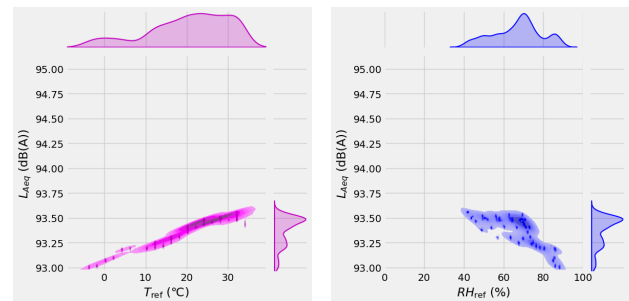
(c) sensor #2
