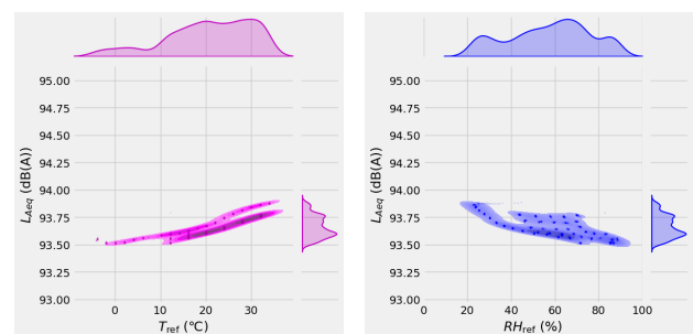
(e) sensor #4
