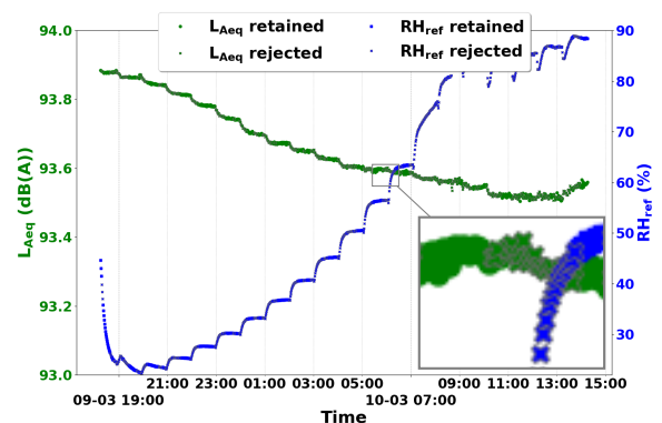
(b) L_{Aeq} (green) vs. RH_{ref} (blue)
