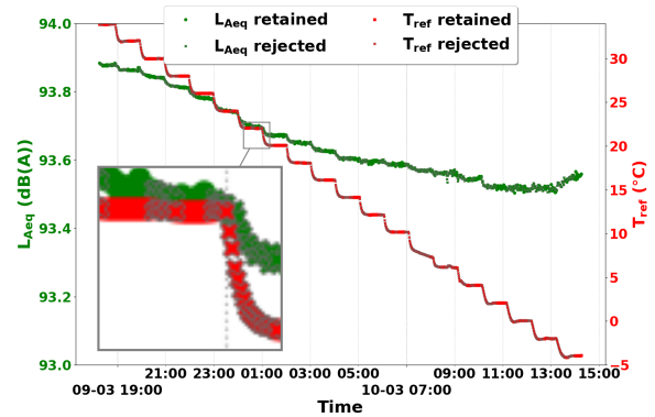
(a) L_{Aeq} (green) vs. T_{ref} (red)
