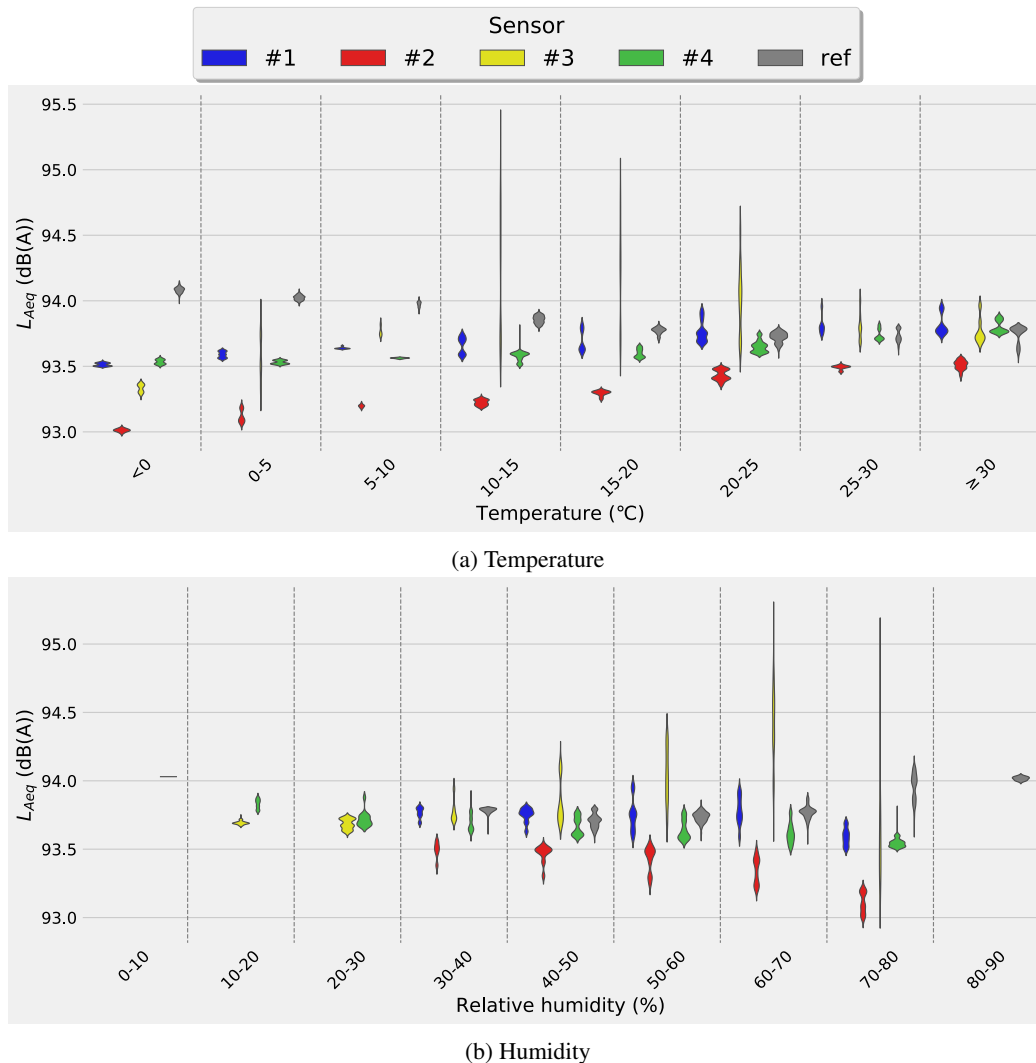
Figure 7: Categorical plots of the L_{Aeq} values according to (a) the temperature and (b) relative humidity for the sonometer and low-cost sensors respectively.
