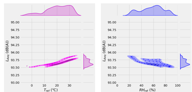
(e) sensor #4
