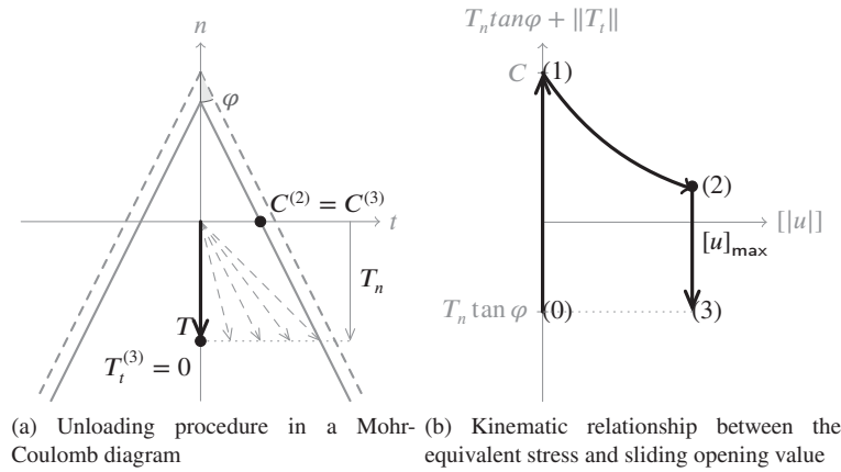
Figure 10: Local constitutive model at the discontinuity interface during the elastic unloading procedure.
