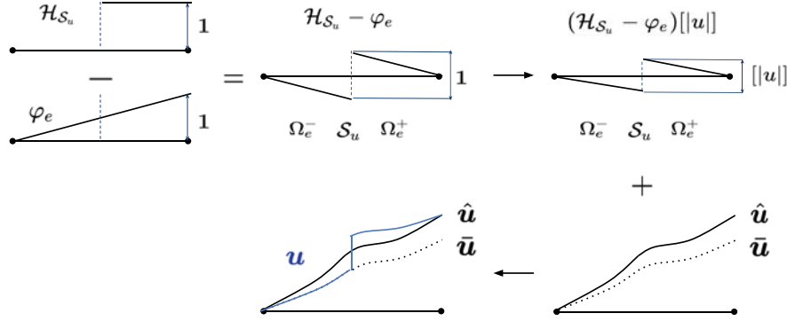
Figure 3: An one-dimension decomposition of the displacement field.
