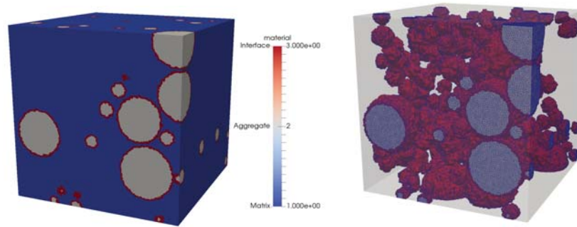
(a) Morphology of the cube with randomly positioned spheres (b) Projection to an unstructured mesh
