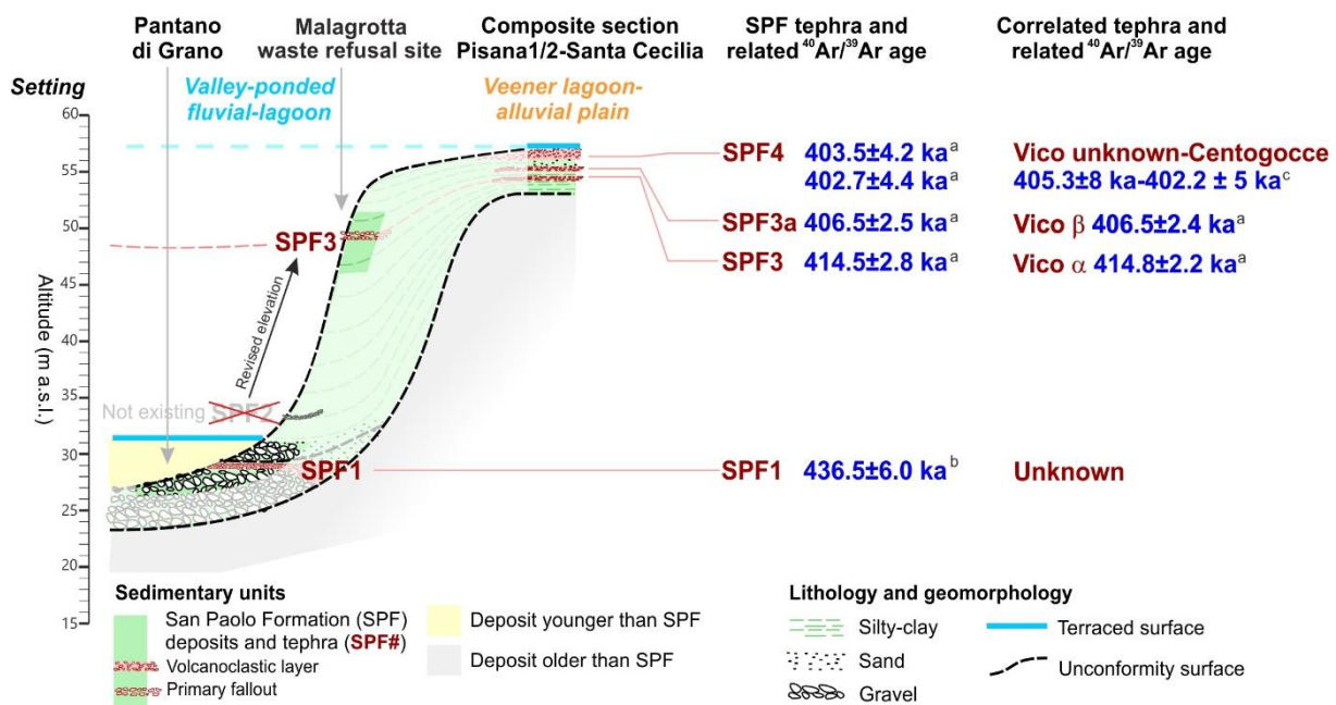
13 14 Figure 3. Sedimentary, geomorphological, and tephrochronological framework of the 15 aggradational succession of San Paolo Formation in Roman coastal area of Ponte Galeria that 16 spans the MIS 12 through MIS 11 glacial-interglacial transition (modified from Pereira et al., 17 2020). The elevation and the age of what was previously referred as SPF2 layer, dated to 18 423.5 \pm 5 ka (Karner and Renne, 1998, sample R94-30C), have been reappraised by Pereira 19 et al. (2020), who demonstrated that it actually matches SPF3 layer, correlated to the Vico \alpha 20 eruption dated by these authors to 414.8 \pm 2.2 ka. Data source; a Pereira et al. (2020); b Marra 21 et al. (2016); c Karner et al., 2001b; Gaeta et al. (2016). All the ages from literature are here
