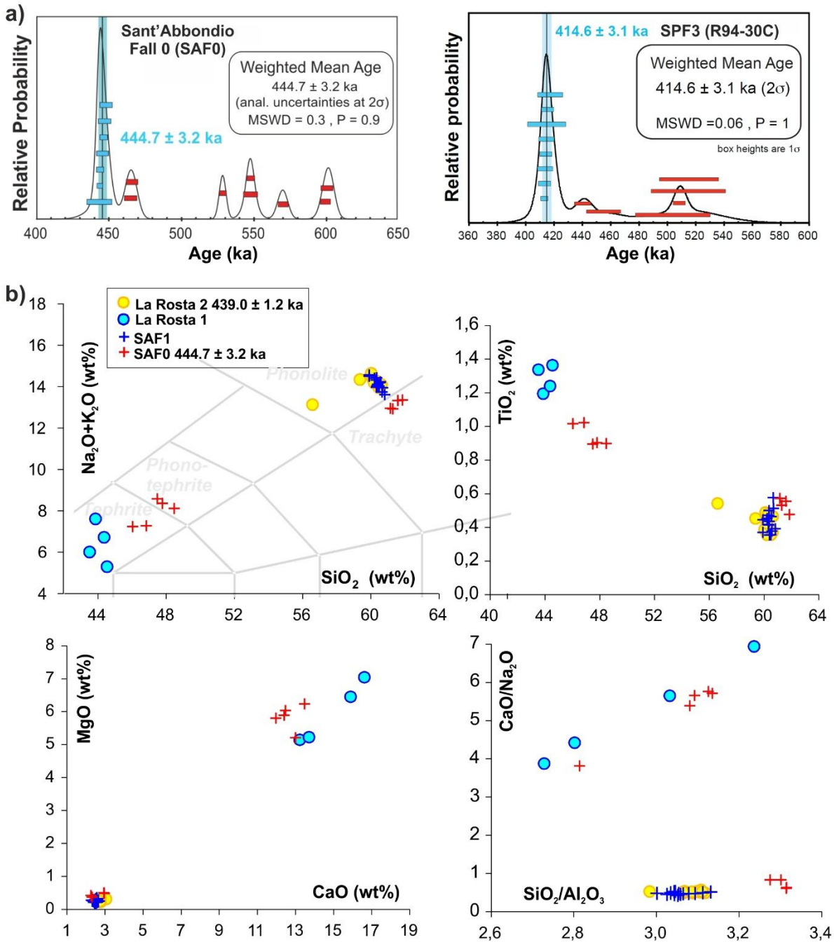
6 7 Figure 6. Age and geochemistry of the investigated tephra layers. a) Single grain ^{40}\text{Ar}/^{39}\text{Ar} 8 age of SAF0 and SPF3 (R94-30C) on single grain presented as probability diagram; b) total
