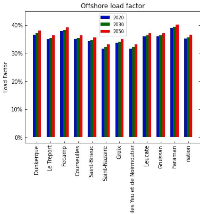
Fig. 12. Annual-average Load factor for various sites where offshore wind farms are planned in France, for the improvement due to advanced hub-height effect in 2030 (green bar) and 2050 (red bar), compared to current status in 2020 (blue), as derived from EPPCF model using ERA5 reanalysis wind speed data for regional and national offshore wind.
