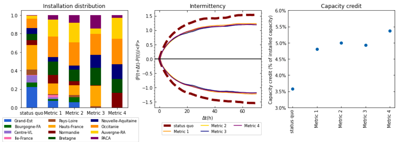
Fig. 8. Results of the optimization of the Onshore wind regional distribution aiming at a reduction of the national production intermittency, based on different metrics (i.e. Metric1: lowest relative wind power change for \Delta t = 1 , Metric2: same as metric1 but for \Delta t = 6 , Metric3: same as metric1 but for \Delta t = 24 , Metric4: highest capacity credit). Left: Regional distribution of the installed capacities for the present and the various criteria. Center: Representation of the intermittency for the current and the optimized distribution. Right: Capacity credit for the current and optimized distributions.
