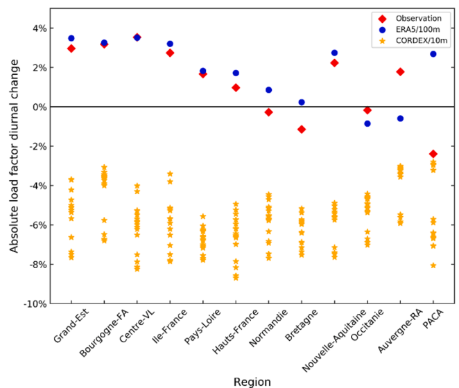
Fig. 17. Comparison of diurnal wind production difference (19 h-6 h compared to 7 h-18 h) among observation data and simulated wind production time series using wind speed of ERA5 at 100 m and multi-ensemble CORDEX models at 10 m.
