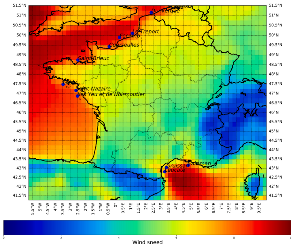
Fig. 10. Annual mean wind speed (ERA5 model) and location of the offshore wind farm projects.
