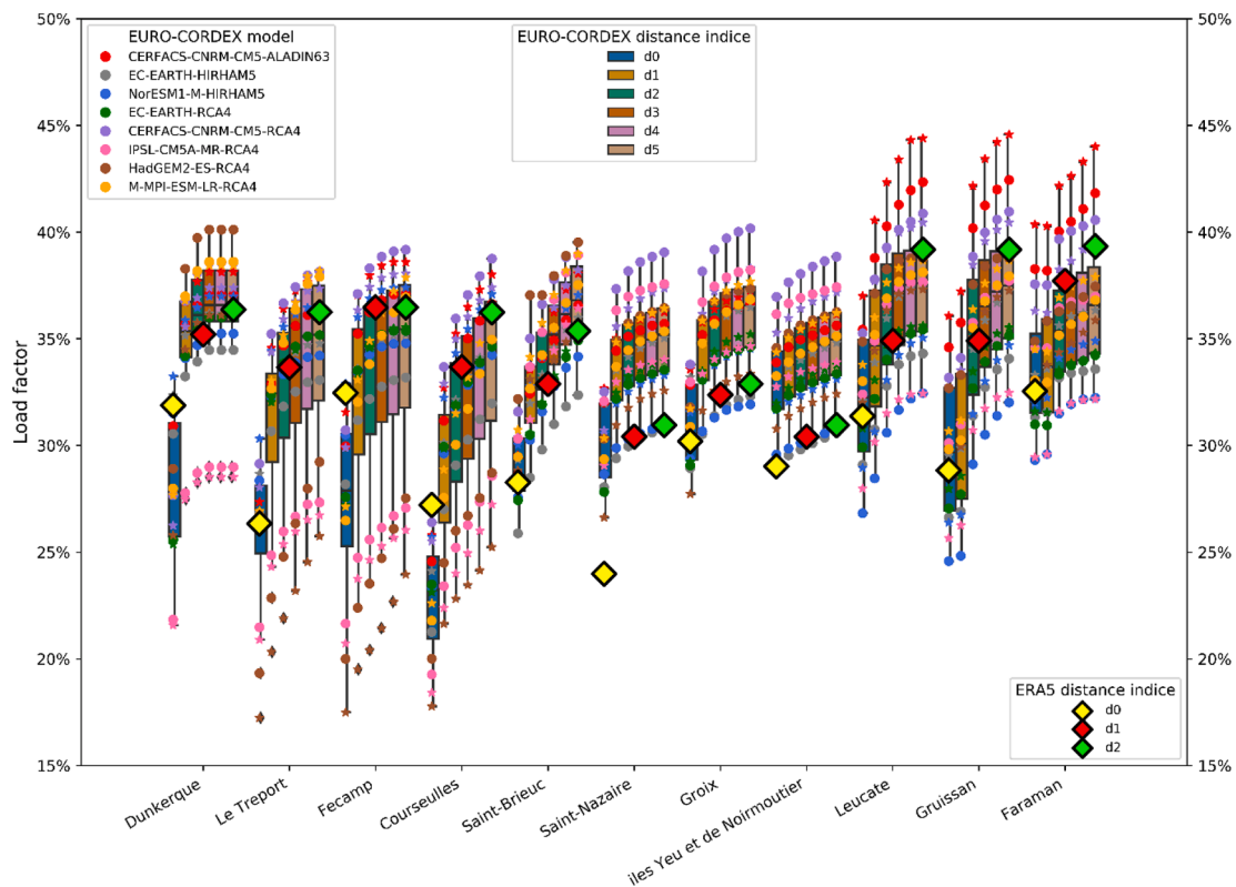
Fig. 11. France offshore wind farm estimated mean load factor under different distances away from the coast in both ERA5 and EURO-CORDEX from 2013 to 2019. d0 marks its original location, d1 marks a location away one times spatial resolution (i.e. 0.11° for EURO-CORDEX model and 0.25° for ERA5) from its original location, d2 marks two times spatial resolution and so on and so forth. The boxplot represents the distribution of the estimated load factor of a wind farm among EURO-CORDEX simulations under RCP4.5 (“*” marker) and RCP8.5 (“o” marker) scenario. ERA5 simulated load factor is represented using diamond marker.
