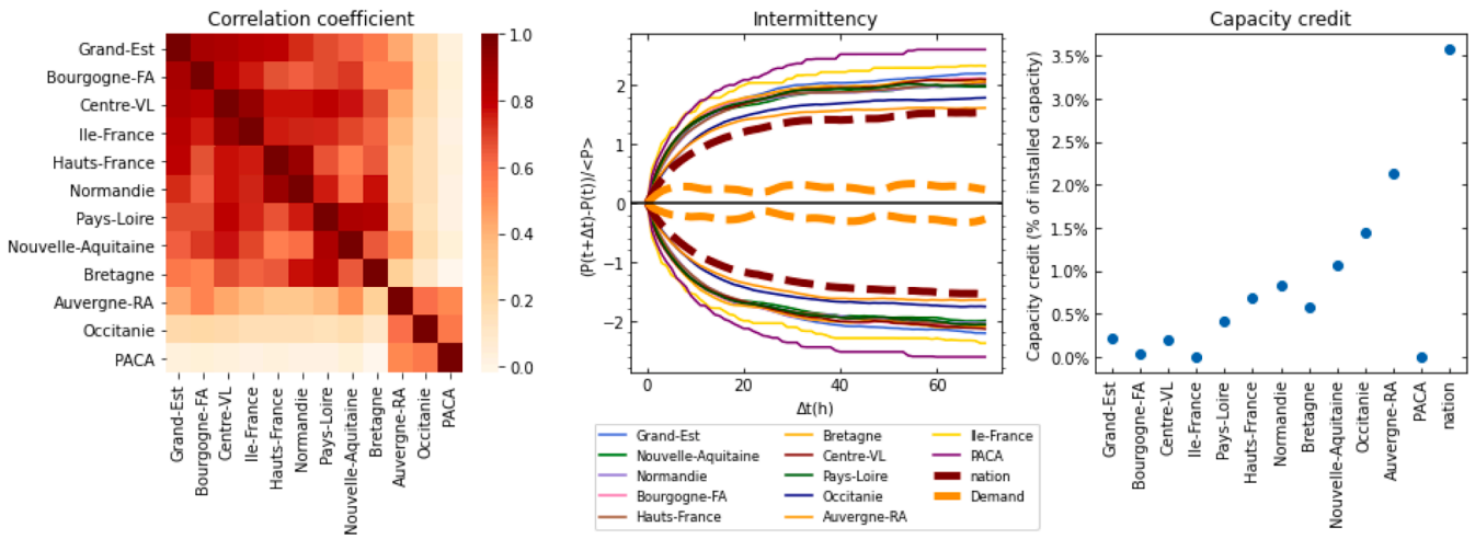
Fig. 7. Onshore wind intermittency and spatial decorrelation current state quantification. Pearson correlation coefficients of onshore wind load factor time series among regions (left). Regional wind load factor (solid line), national wind load factor (dashed line in darkred) and national demand (dashed line in orange) intermittency quantification with regard to rapidity and amplitude of wind power variation; namely, the 5th and 95th percentile of relative wind load factor or demand change relative to average wind load factor or demand at intervals ( \Delta t ) from 1 h to 70 h (center). Regional and national onshore intermittency quantification with regard to equivalence of ‘firm’ capacity in long-term system planning; namely, the capacity credit measured by the average load factor exceeding 95th percentile over top 10% load periods (right). The data is based on hourly historical observations from 2013 to 2019 provided by RTE.
