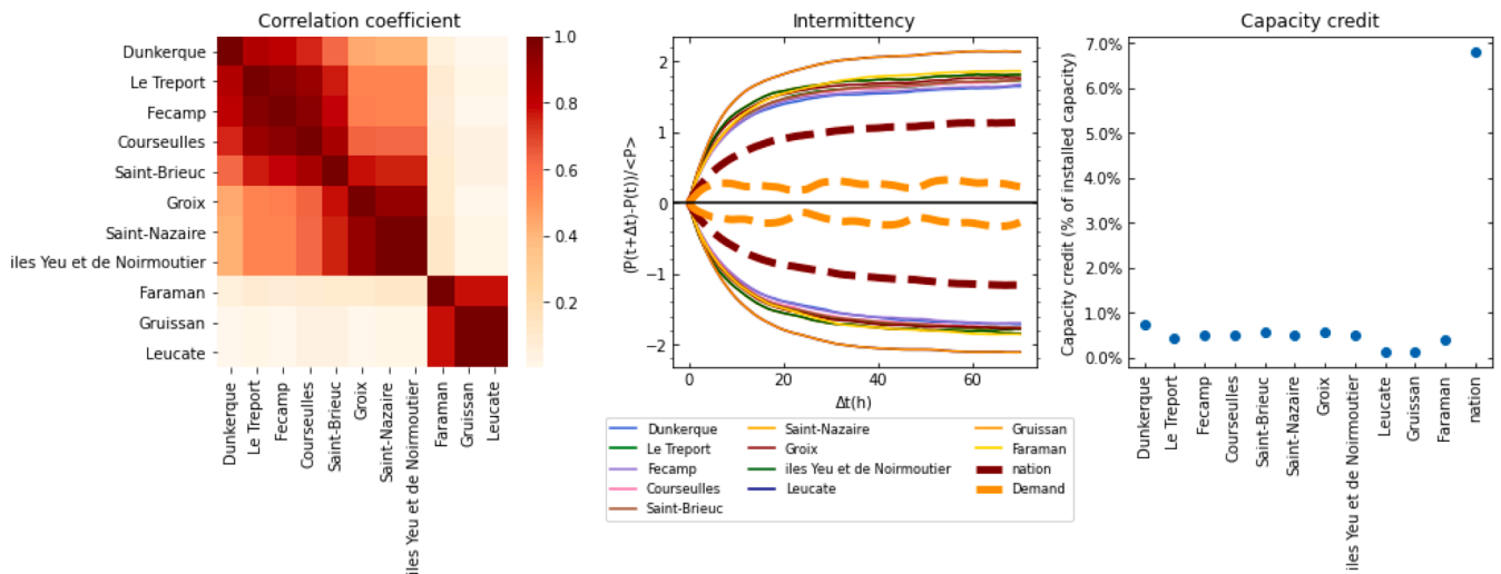
Fig. 13. Same as Fig. 5 but for the Offshore wind projects. The data used is based on simulation result in using EPPCF method applying ERA5 wind speed data from 2013 to 2019.
