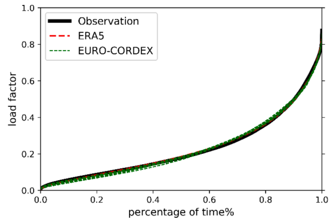
Fig. 4. The cumulative distribution of observed (black solid line) and simulated national load factor (dash line) for the year of 2013–2019.
