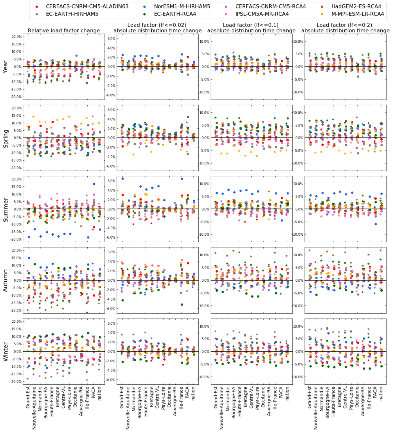
Fig. 15. Regional and national onshore wind relative mean load factor change & absolute distribution time change (i.e. the absolute change of percentage of time when the load factor is inferior to 2%, 10% and 20%) during one future (2045–2055) and one historic (2006–2015) period for annual and 4 different seasons. The colored star markers mean for RCP4.5 (left line), the circle markers mean for RCP8.5 (right line).
