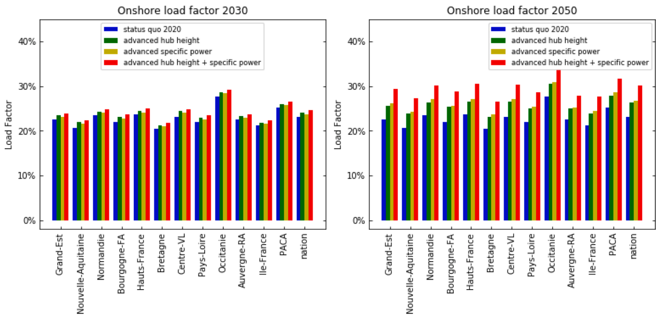
Fig. 6. Load factor improvement including advanced hub-height effect (green bar), advanced specific power effect (yellow), and combined effects of hub-height and specific power improvement (red), compared to current status in 2020 (blue), as derived from EPPCF model using ERA5 reanalysis wind speed data for regional and national onshore wind in 2030 (left), and 2050 (right).
