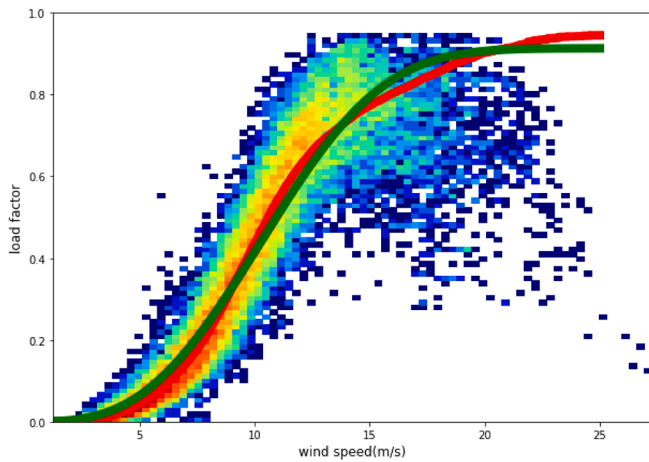
Fig. 9. Comparison of the observed and modeled load factor for offshore wind power off the coast of Germany. The colored scatterplot is a density histogram of reported load factor and ERA5 wind speed at 100 m for the year of 2016–2018; the red curve is the derived EPC by matching the wind speed and load factor CDF; the green curve is the EPPCF method obtained through the best fit procedure.
