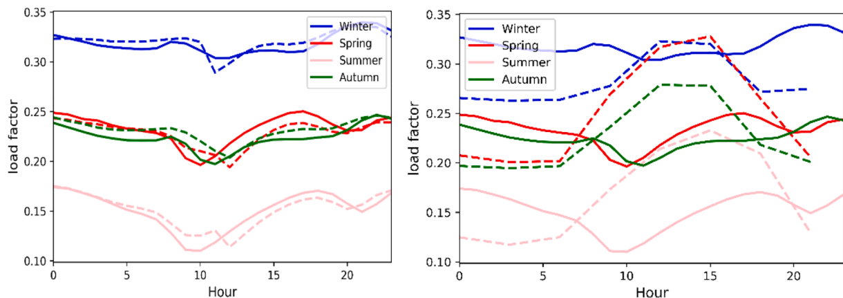
Fig. 5. France national onshore wind power seasonal-diurnal validation of ERA5 (left) and CERFACS-CNRM-CM5-ALADIN63 RCP4.5 as an example of EURO-CORDEX model (right). The dash lines and solid lines are observed and simulated respectively from 2013 to 2019.
