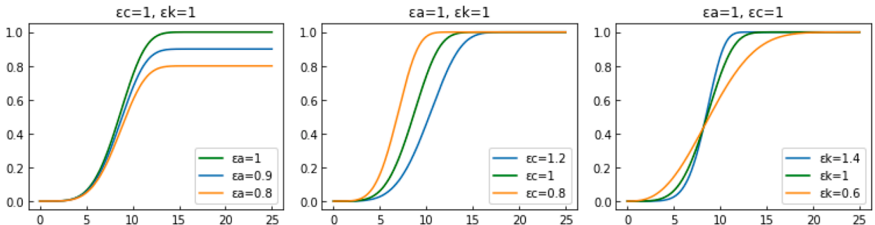
Fig. 2. Impact on the theoretical power curve functions when one parameter is changed and the others are kept to the nominal value of 1.
