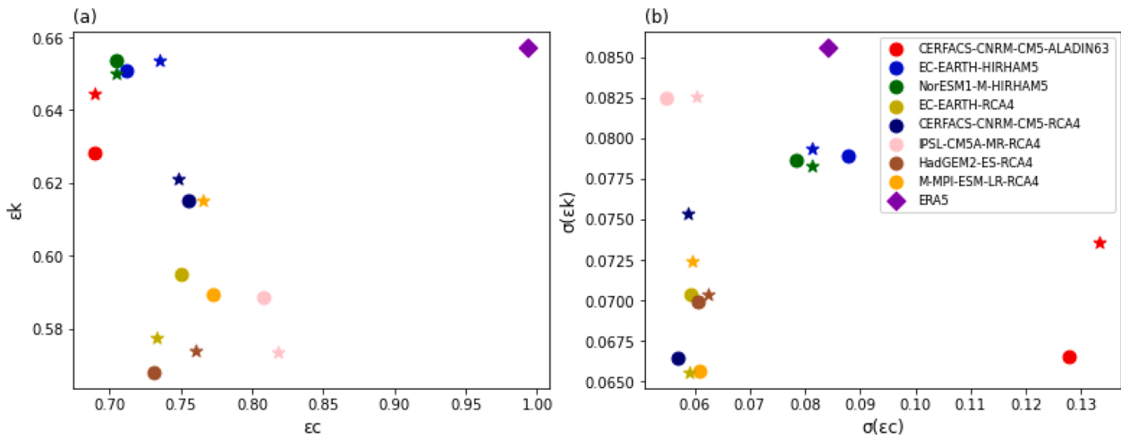
Fig. 16. Comparison of mean (a) and standard deviation (b) of the power curve coefficients, derived from the EPPCF model. The two figures compare the difference among different models across all regions, “*” star markers mean for EURO- CORDEX scenario RCP4.5, circle markers mean for EURO-CORDEX model scenario RCP8.5, diamond star markers in purple mean for ERA5.
