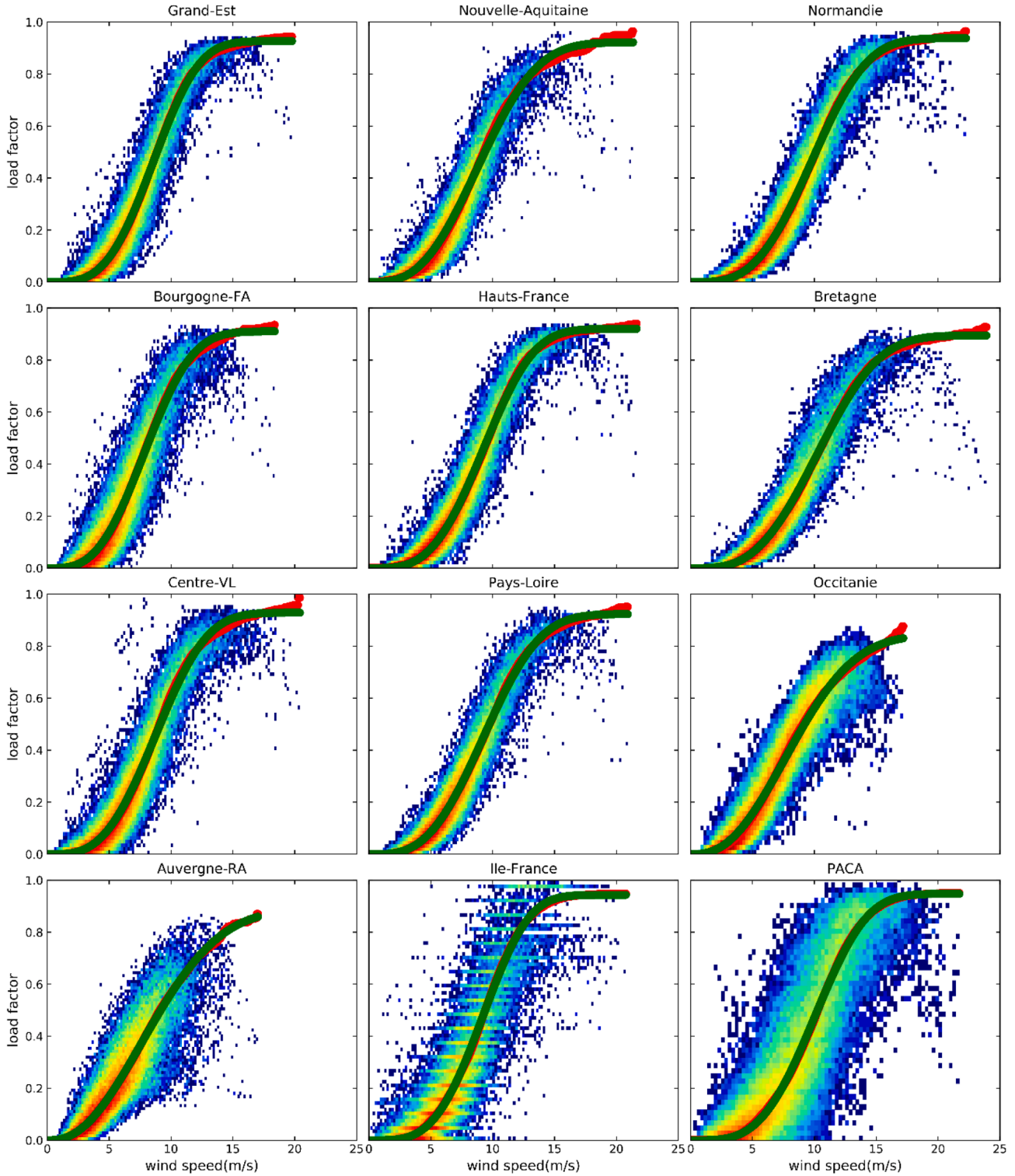
Fig. 3. France onshore wind power curve hourly validation by region. The density histogram shows the ERA5 wind speed at 100 m for the year of 2013–2019 together with the regional wind load factor provided by RTE. The red curve is the EPC derived by matching the wind speed and load factor CDF, whereas the green curve is the fitted curve of EPC using EPPCF method.
