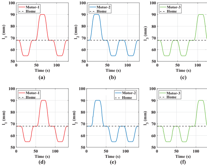
FIGURE 9. Position of prismatic springs along the linear trajectory for two springs pull experiment in the (a),(b),(c): vertical and (d),(e),(f): horizontal orientations of the mechanism
