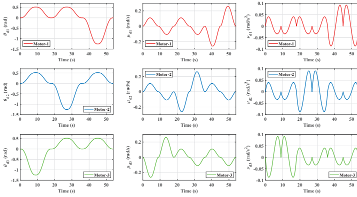
FIGURE 4. Theoretical angular positions ( \theta_d ), velocities ( \mu_d ) and accelerations ( \nu_d ) of the pulleys of Motor-1 (red), Motor-2 (blue) and Motor-3 (green) for one spring pull experiment
