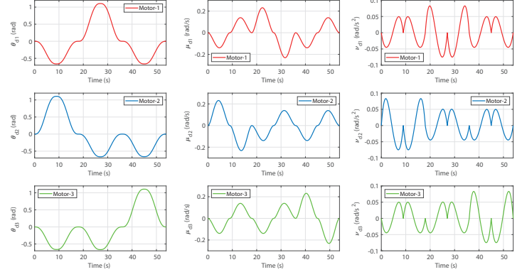
FIGURE 5. Theoretical angular positions ( \theta_d ), velocities ( \mu_d ) and accelerations ( \nu_d ) of the pulleys of Motor-1 (red), Motor-2 (blue) and Motor-3 (green) for two springs pull experiment
