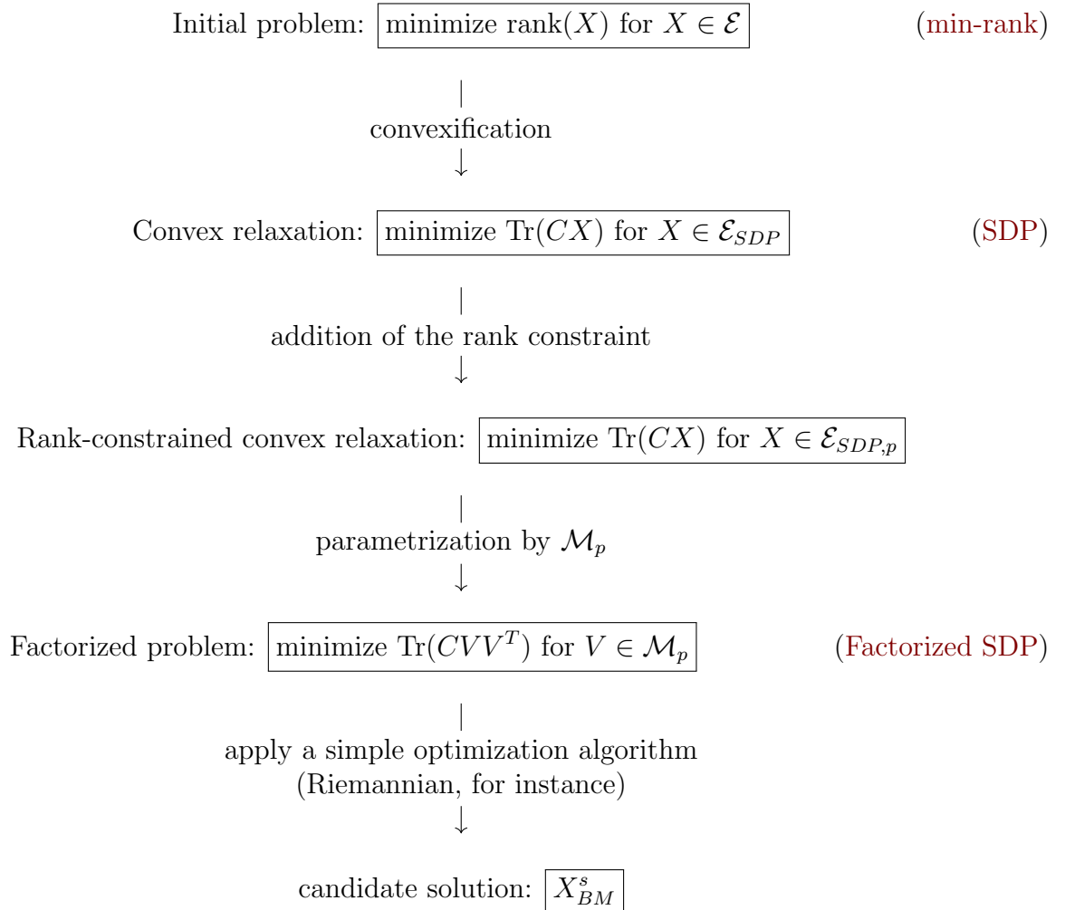
Figure 4: Schematic view of a Burer-Monteiro method
