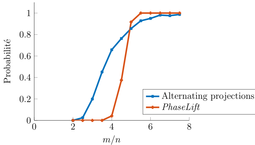
Figure 1: Success probability for two phase retrieval algorithms, as a function of m/n , for n = 40 .
