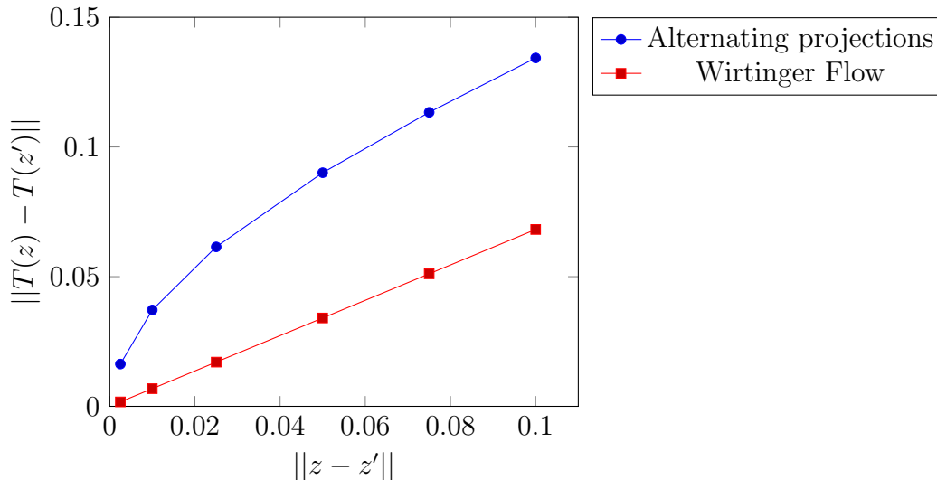
Figure 3: \mathbb{E}\|T(z) - T(z')\| as a function of \|z - z'\| for two phase retrieval algorithms, Wirtinger Flow and alternating projections, for the reconstruction of signals with dimension n = 400 from m = 4000 phaseless measurements. For any distance \|z - z'\| , \mathbb{E}\|T(z) - T(z')\| is computed by averaging over 1000 random pairs (z, z') .
