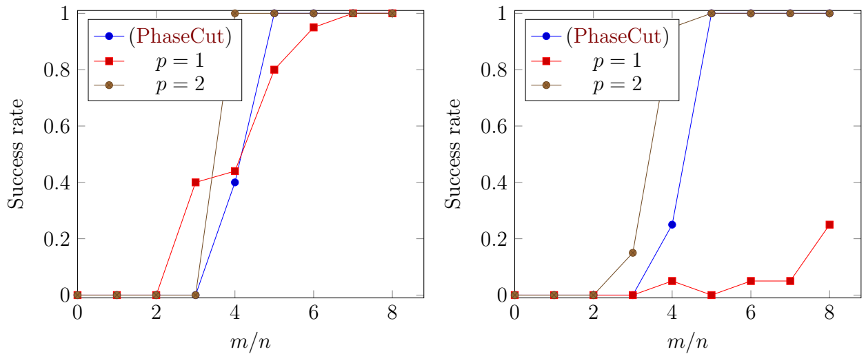
Figure 5: Success rate, as a function of m/n , for three algorithms: (PhaseCut), a Burer-Monteiro method with p = 1 , a Burer-Monteiro method with p = 2 . The signal dimension is n = 32 . The figure on the left corresponds to measurement vectors independently chosen according to normal laws and the figure on the right to measurement vectors representing a “wavelet transform”. Success rates have been computed by averaging the results of 20 reconstruction attempts.
