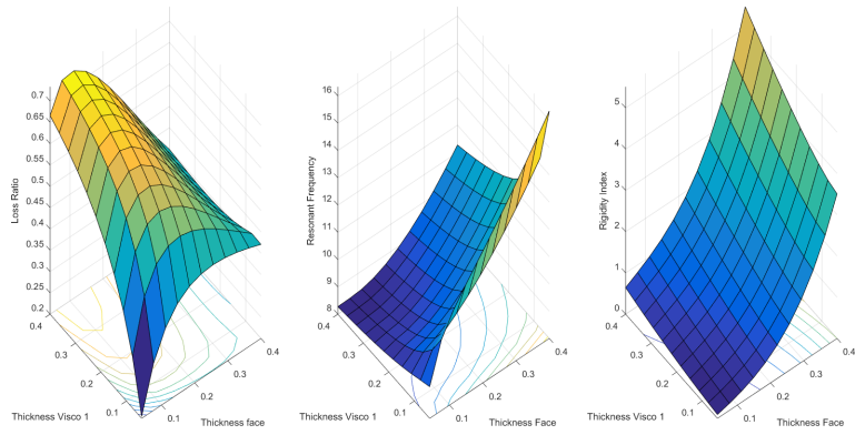
Figure 6: Evolution of loss ratio, resonant frequency and rigidity index versus X_1, X_2 for X_3 = 0.28
