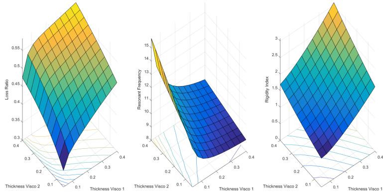
Figure 5: Evolution of loss ratio, resonant frequency and rigidity index versus X_2, X_3 for X_1 = 0.28
