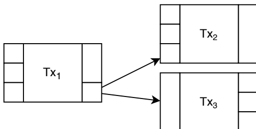
Figure 1: T_{x_2} uses the first output of T_{x_1} as its third input. Hence, T_{x_2} depends on T_{x_1} and must appear after it in the chain. In practice, T_{x_2} has a pointer to T_{x_1} but for demonstration purposes, we found it more convenient to show this as an arrow that models the flow of value from T_{x_1} 's output to T_{x_2} 's input.
