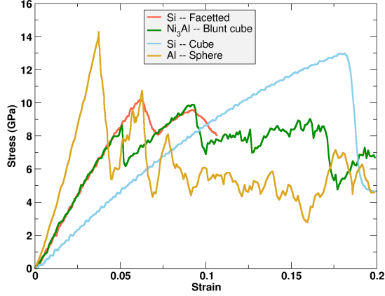
FIGURE 4. Compressive stress as a function of strain for MD nanocompression simulations of various NPs, retrieved from the literature (True stress: red curve [56], light blue curve [56], gold-enrod curve [84]). Engineering stress: green curve [54]).
