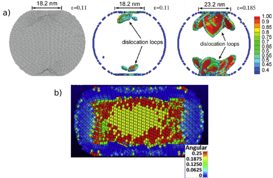
FIGURE 9. Si NPs compressed using MD simulations. a) 40 nm spherical NP deformed at 11% (left and middle image) and 18.5% (right image), showing the homogeneous nucleation and expansion of dislocation loops (slip vector representation) in the vicinity of the contact surfaces (adapted from [131] with permission). b) Formation of a \beta -tin phase (yellow atoms) in the center of a 10 nm spherical NP after unloading following a \langle 100 \rangle compression (adapted from [92] with permission).
