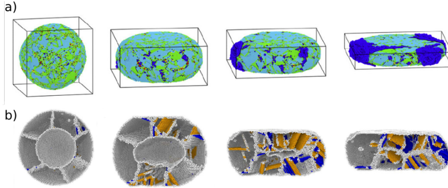
FIGURE 13. a) 20 nm polyethylene nanospheres ( \text{CH}_x beads in blue) coated with a 0.5 nm thick Ni layer (green atoms), at different compression (Adapted from [168] with permission). b) Cross-section views of polycrystalline hollow 20 nm Pd nanoparticles with a grain size of 10 nm and a shell thickness of 5 nm, at different compression strains. White atoms correspond to the grain boundary region, and the inner/outer surfaces. Orange and blue atoms depict atoms belonging to SF and twin boundaries, respectively (Adapted from [170] with permission).
