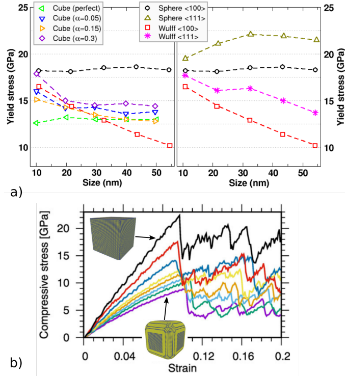
FIGURE 6. a) Maximum stress as a function of size for silicon NPs, for different shapes and orientations (adapted from [56] with permission). \alpha is the rounding coefficient applied to the particle edges and corners ( \alpha = 0 for a perfect cube, and \alpha = 1 for a sphere). b) Stress–strain curves associated with the compression of \text{Ni}_3\text{Al} cubic NPs, with \alpha increasing from the top curve to the bottom one (adapted from [54] with permission).
