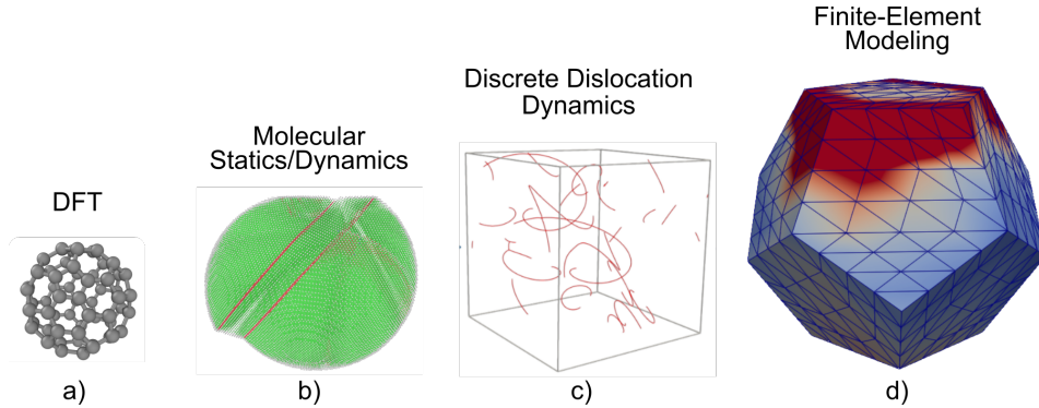
FIGURE 1. Simulation methods currently used to model nanoparticle mechanics with typical examples including a) DFT simulations of the compression of a C_{60} molecule, b) Nanocompression of a Ni NP using atomistic simulation (atoms in FCC environment are colored in green, HCP atoms in red), c) DDD simulation of a MgO nanocube under compression and d) Von Mises stress distribution during the compression of a dodecahedron metal nanoparticle using FEM.
