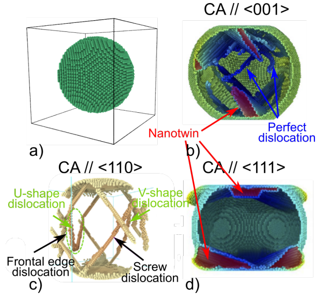
FIGURE 8. BCC niobium nanoparticle under compression using MD, a) Perfect 10 nm diameter niobium nanoparticle, b-d) Elementary deformation processes occurring during compression with compression axis (CA) along \langle 001 \rangle , \langle 110 \rangle and \langle 111 \rangle respectively. Perfect crystal atoms are removed for a sake of clarity. Adapted with authors permission from the work published in Ref. [102].
