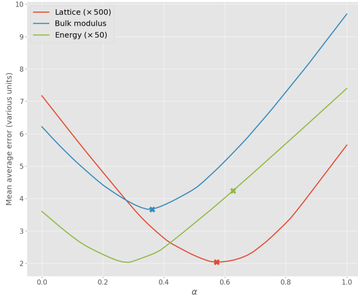
Figure 2. Variations of mean average error (MAE) for three 3C-SiC quantities, with corrections using a weight factor \alpha ranging from 0 to 1 and Eq. 4, using data reported in Ref. [17]. The crosses show the MAE with corrections using \alpha computed using Eq. 2. Values for lattice parameter (cohesive energy) were multiplied by 500 (50) for the sake of comparison.
