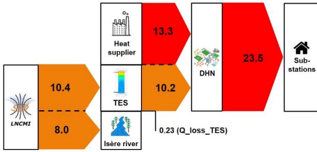
Figure 10a. Sankey diagram (energy flows in GWh/year) for the optimized operation of the WHRS with a source-oriented, energy-based optimal design (i.e. waste heat at 85 °C, and no heat pump). This design is also supported by the exergy-based optimization.
