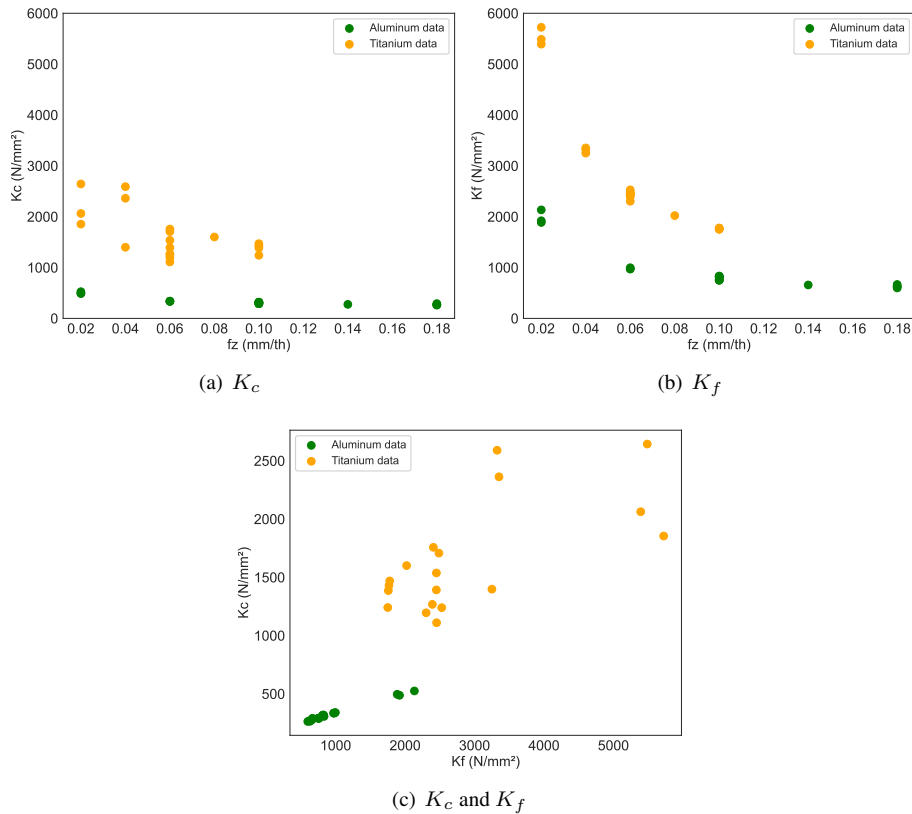
Figure 8: Identification map with K_c per K_f for both materials
