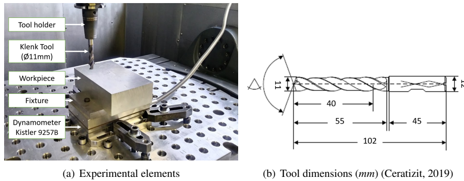
Figure 1: Experimental setup
