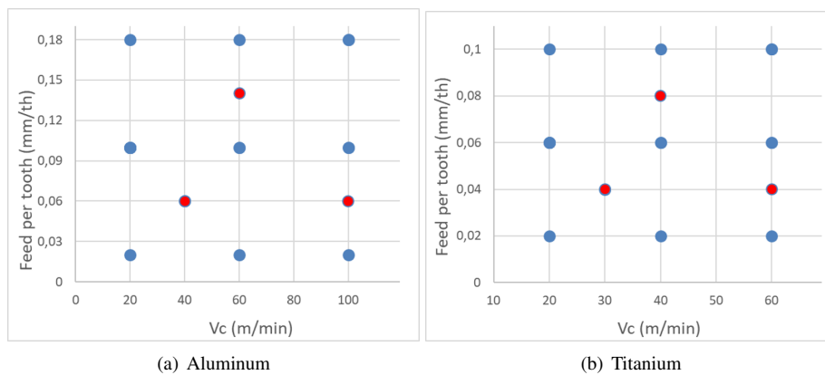
Figura 2: DOE workspace
