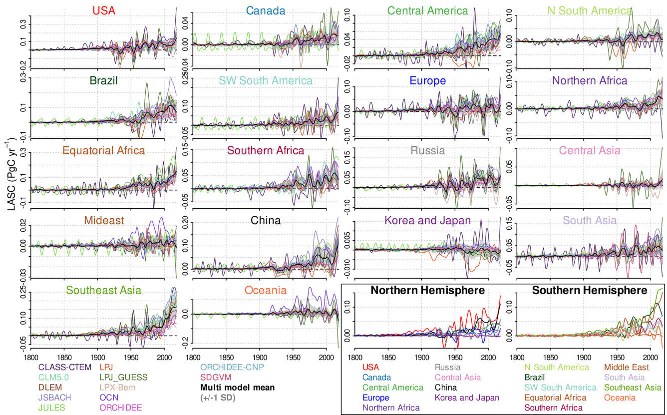
Figure A4. Region-wise smoothed annual loss of additional sink capacity (LASC) in the investigated DGVMs from 1800 to 2018, derived according to Eq. (4). For discussion of individual models refer to Sect. A1. The last two panels show regional ensemble means on a uniform scale.
